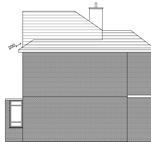
PROPOSED LEFT SIDE ELEVATION
