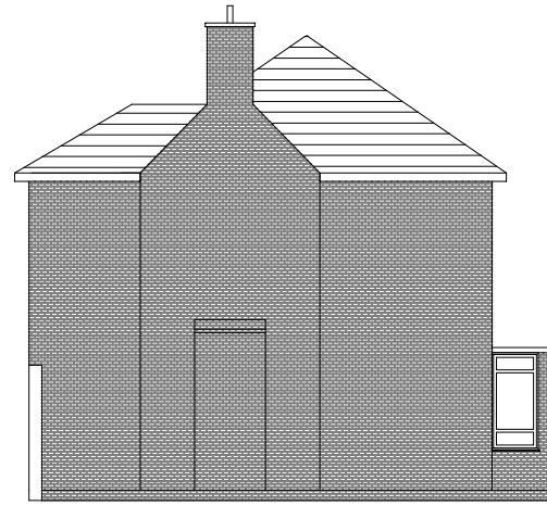
EXISTING RIGHT SIDE ELEVATION
