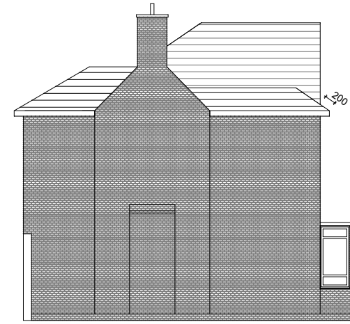
PROPOSED RIGHT SIDE ELEVATION
