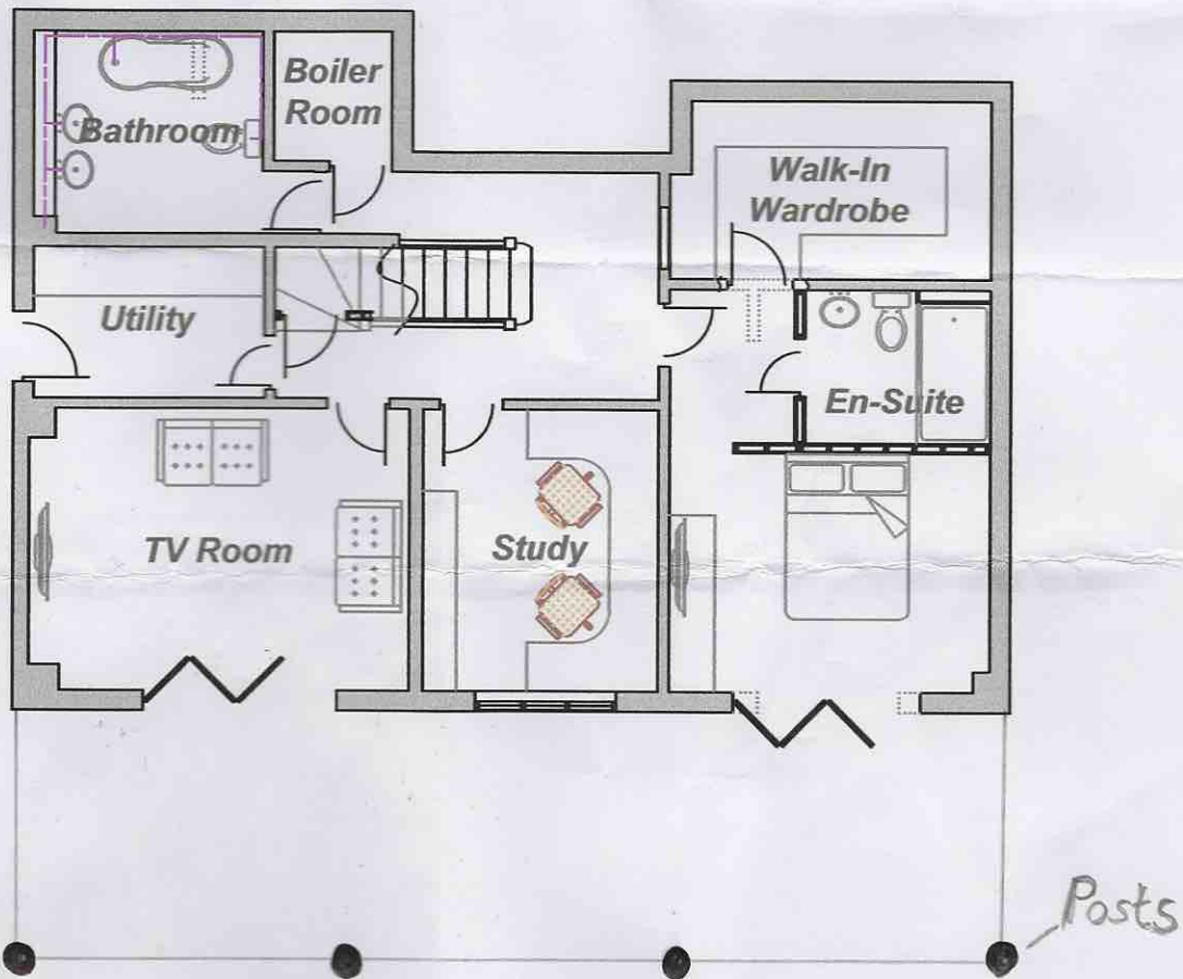
PROPOSED SEMI BASEMENT FLOOR PLAN - 1:100
