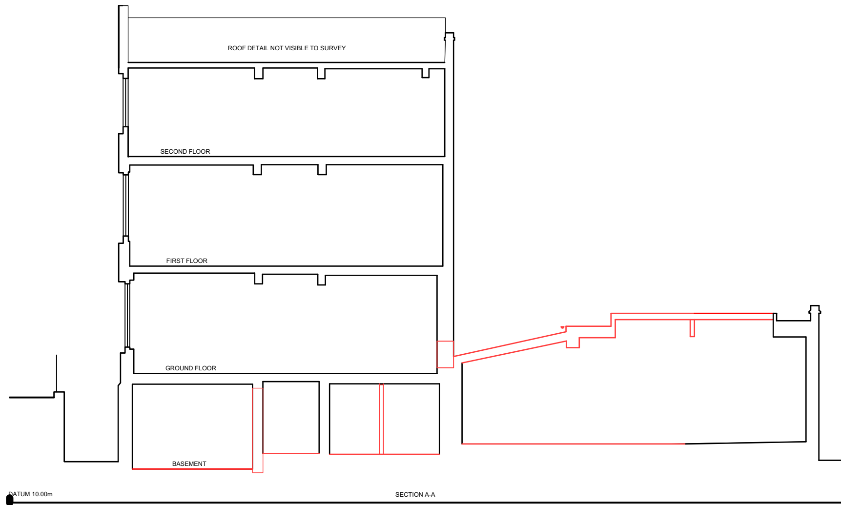
existing section
