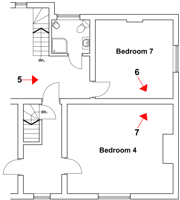
Existing Second Floor Plan (with key to Photographs)
