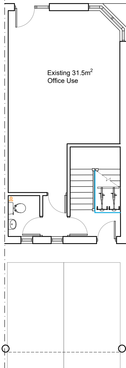
Proposed Ground - 1:100
