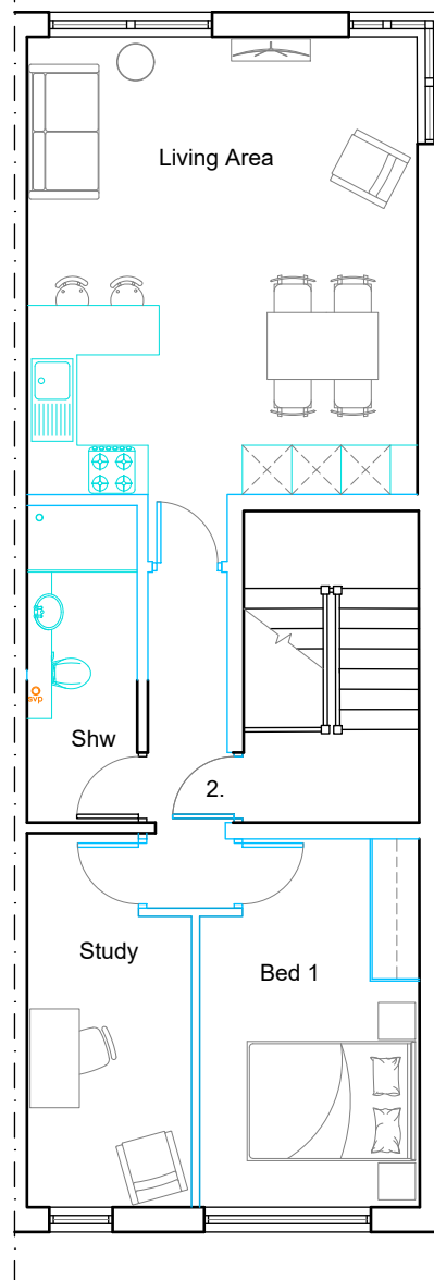
Proposed Second - 1:100
