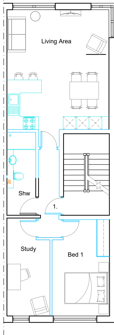
Proposed First - 1:100
