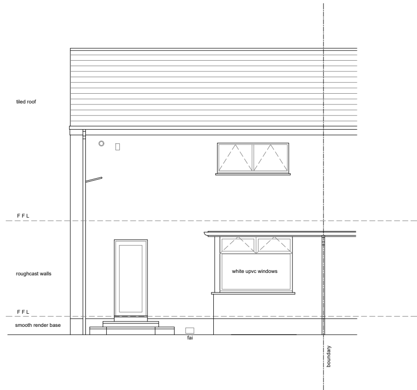
Front Elevation
