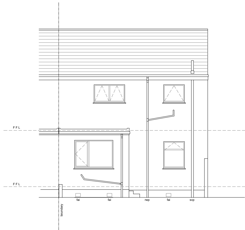
Rear Elevation
