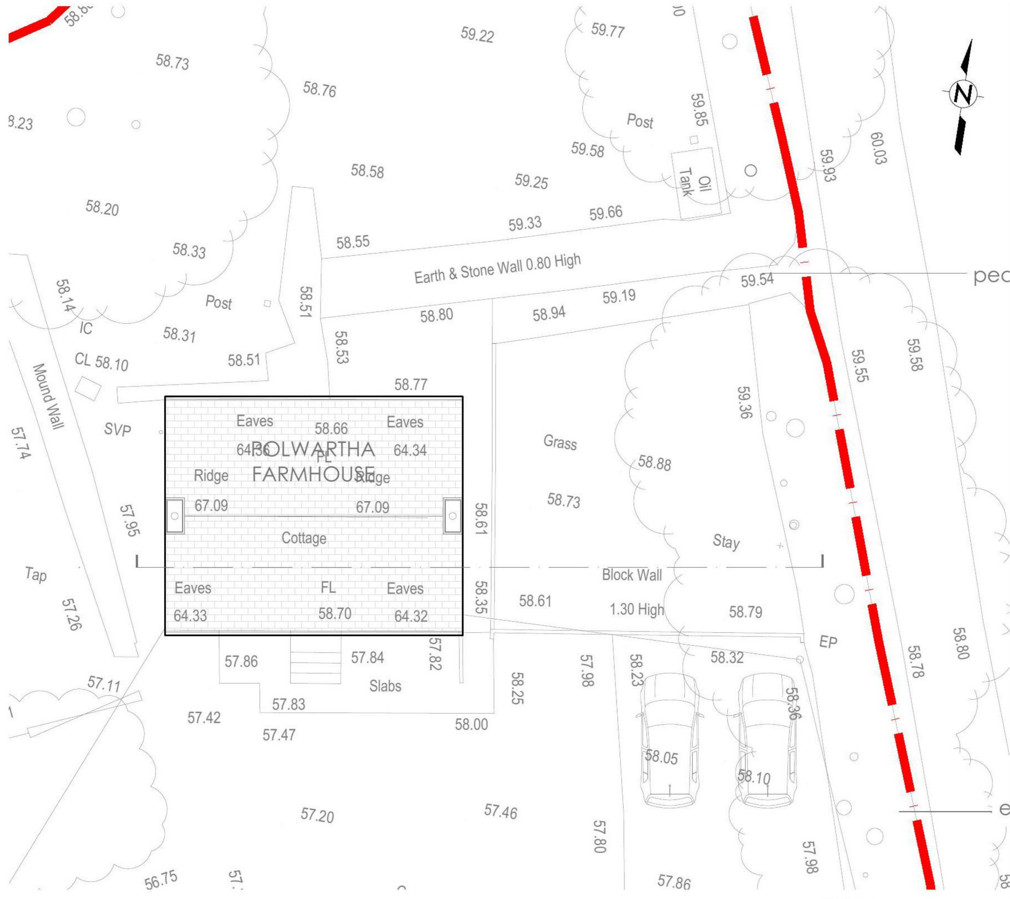
Existing Roof Plan 1:100
