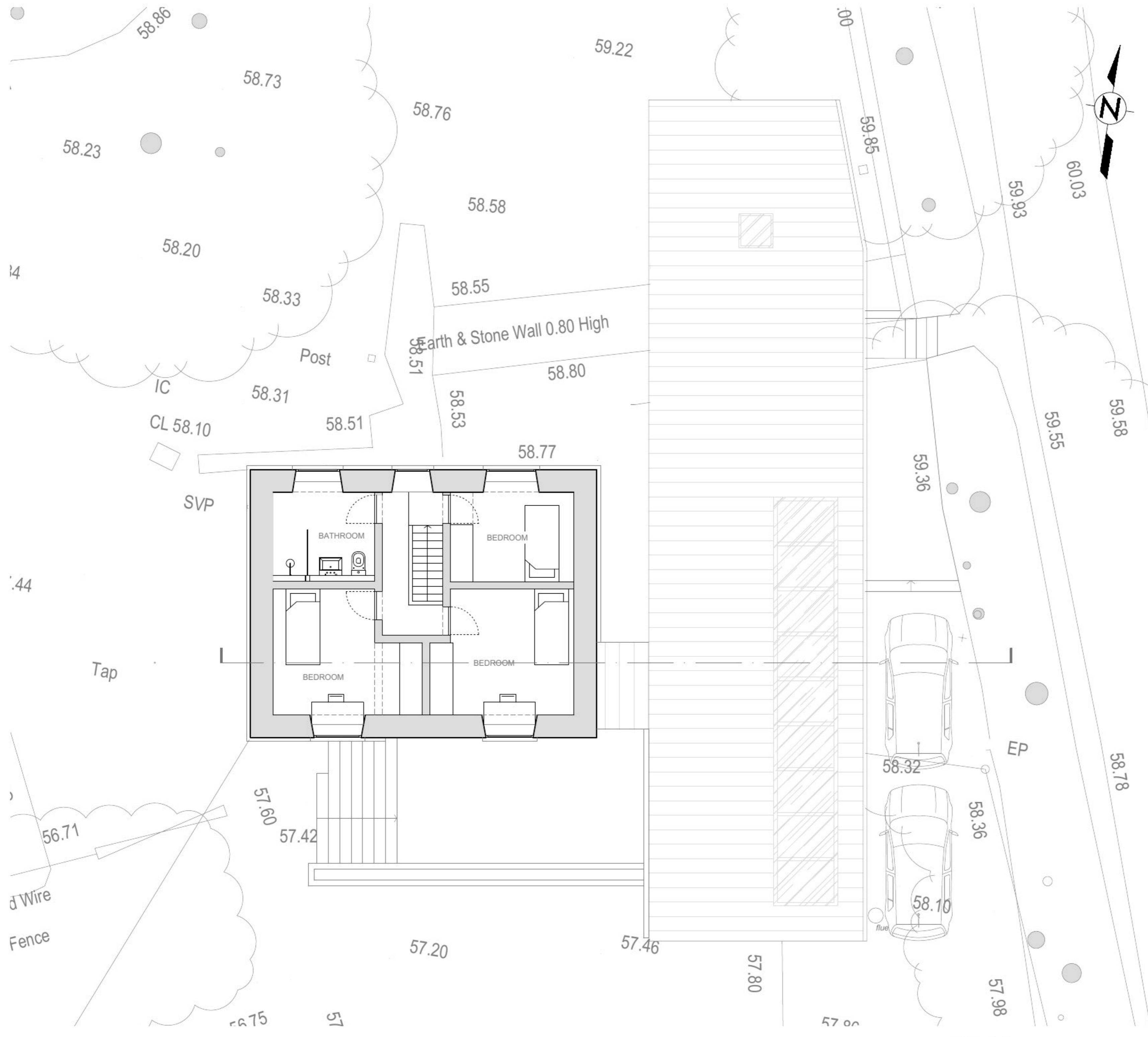
Proposed First Floor Plan 1:100
