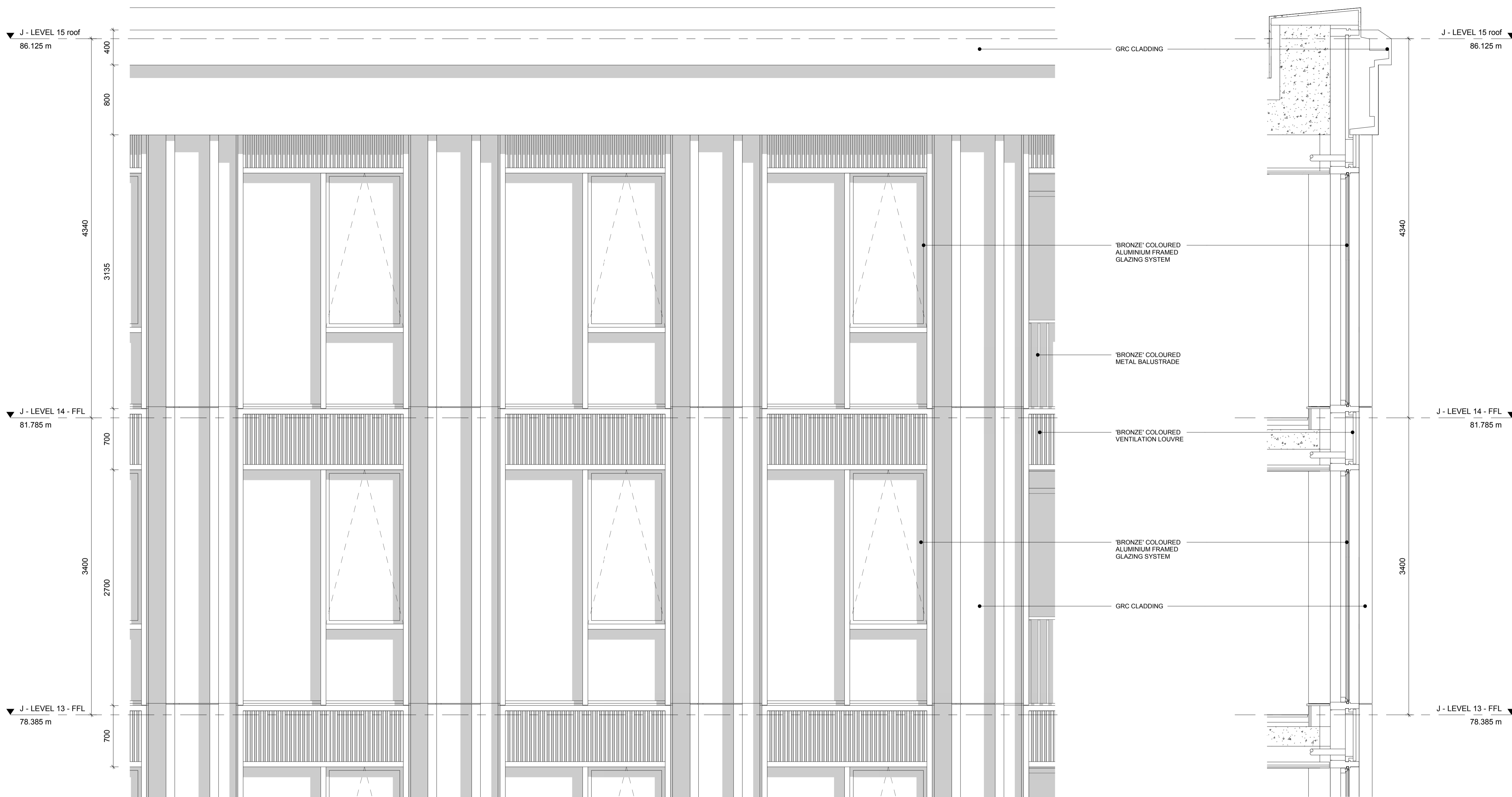
1 Block J - Bay Study 05 - Elevation 1 : 25
