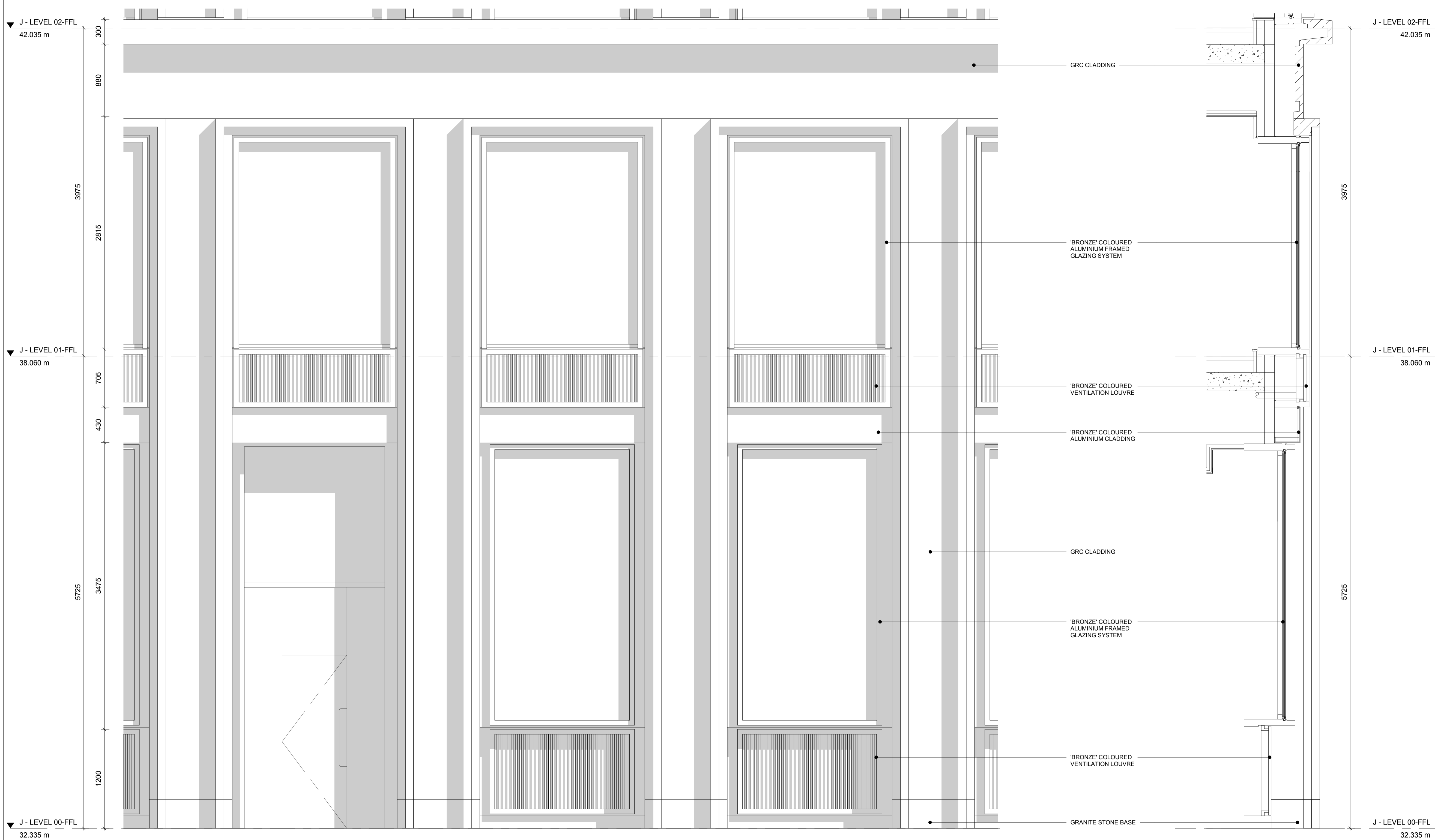
1 Block J - Bay Study 01 - Elevation 1:25
