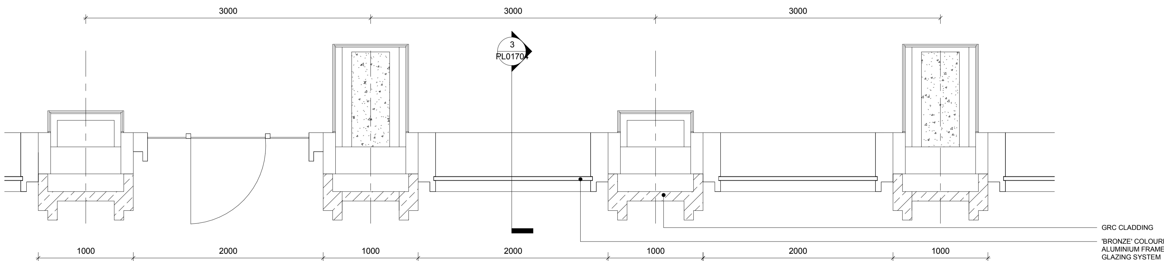
2 Block J - Bay Study 01 - Plan 1:25
