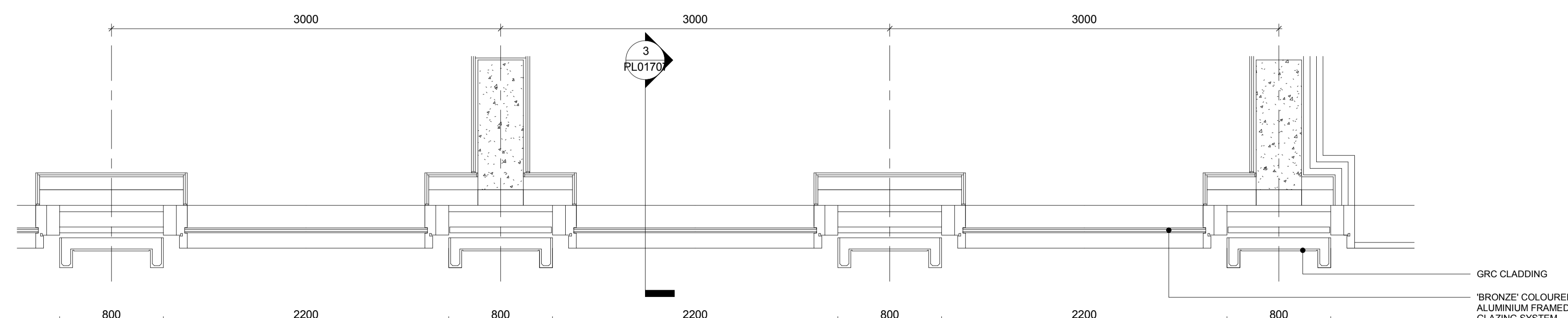
2 Block J - Bay Study 04 - Plan 1:25
