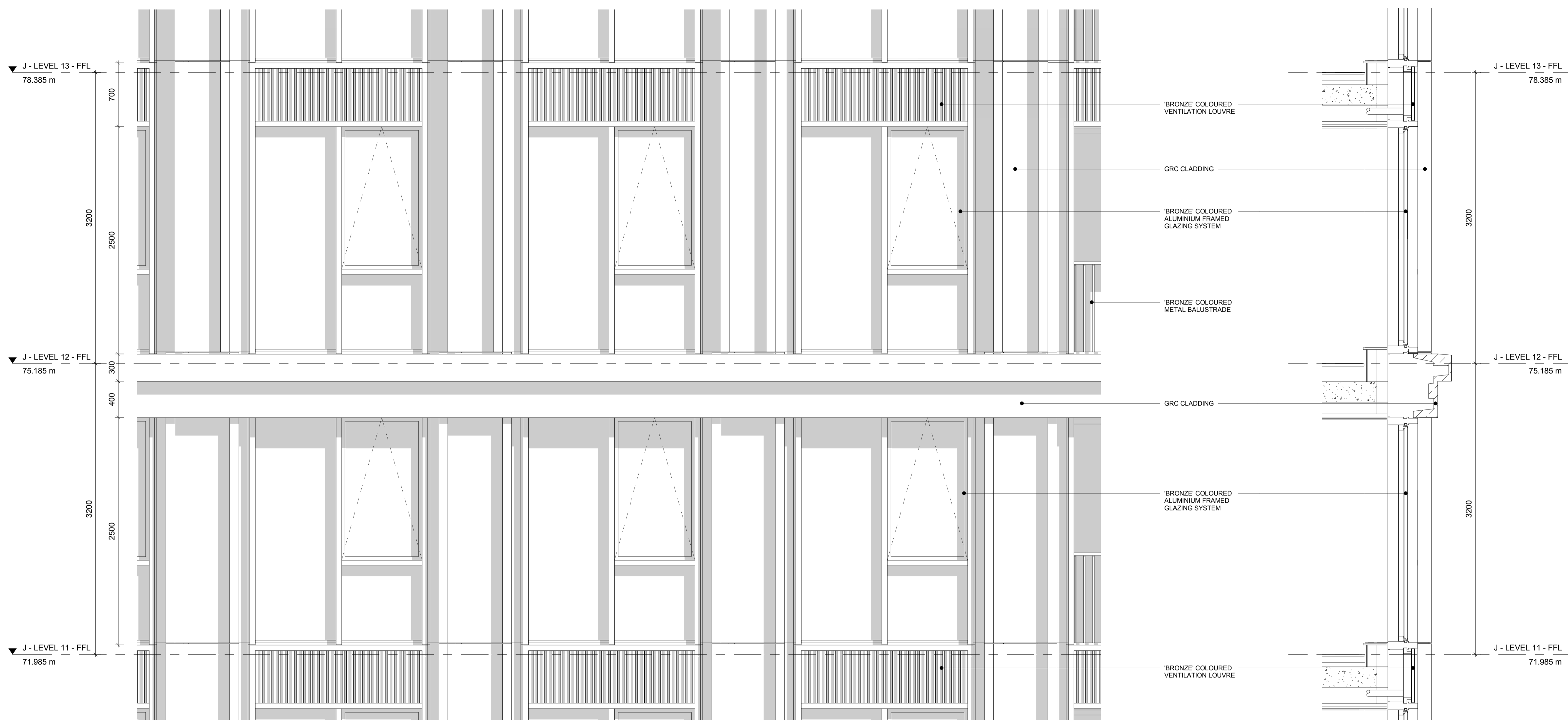
1 Block J - Bay Study 04 - Elevation 1:25
