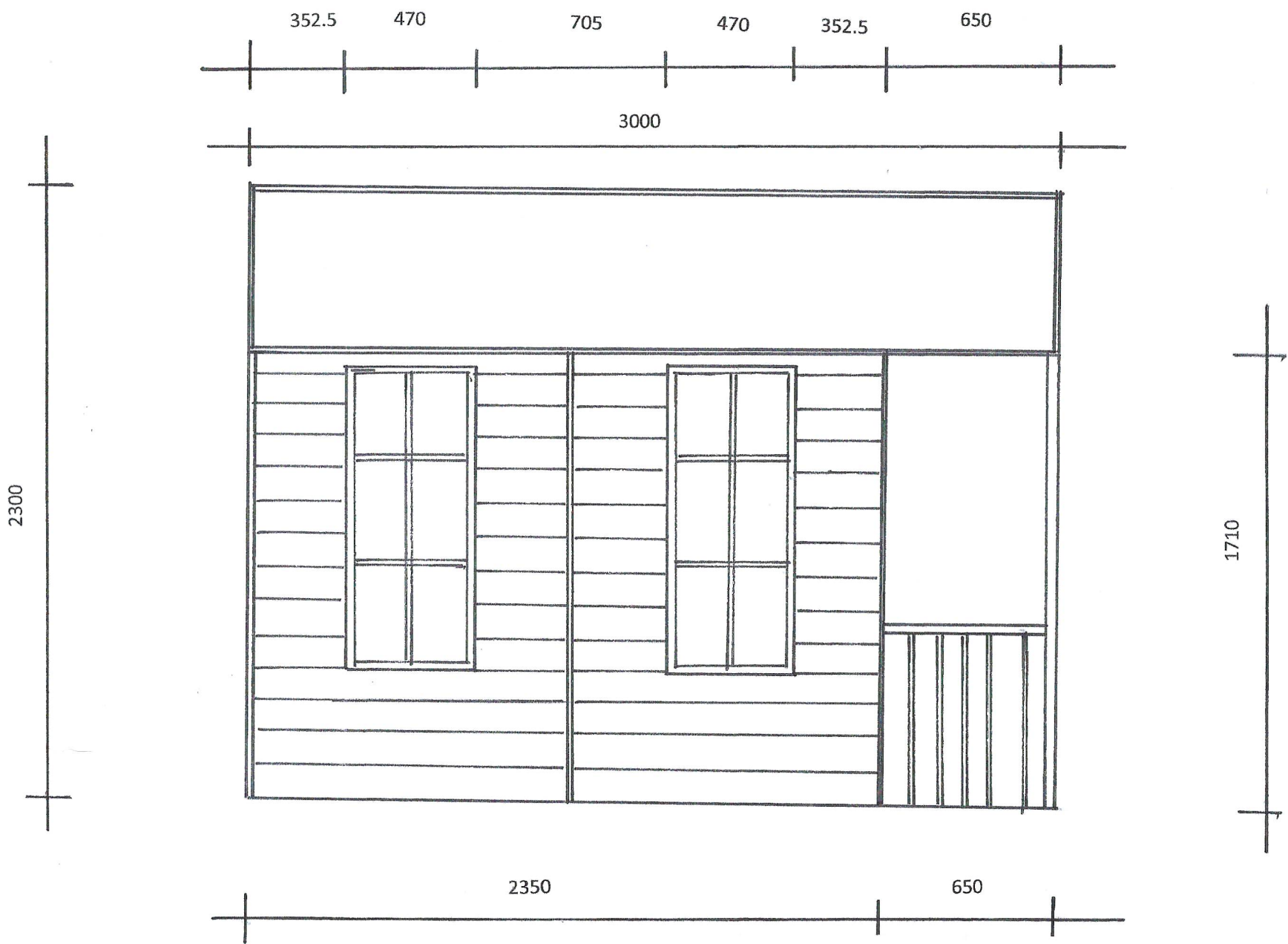
PROPOSED WORKS TO REAR GARDEN AT 1 DOUGLAS AVENUE, GIFFNOCK SUMMERHOUSE (AREA B) - SIDE ELEVATION (WEST) Scale 1 : 20 Date April 2021 Drawing 24
