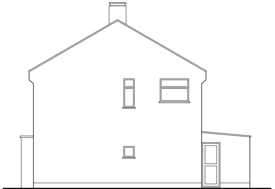
EXISTING SOUTH SIDE ELEVATION
