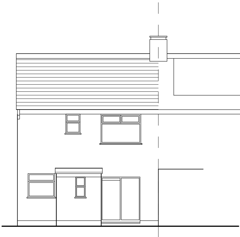
EXISTING REAR SIDE ELEVATION
