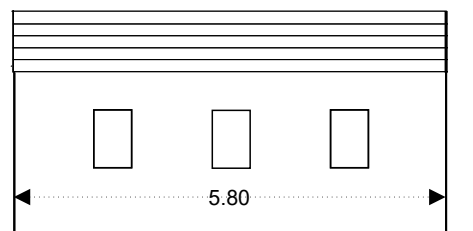
EXISTING NORTH SIDE ELEVATION
