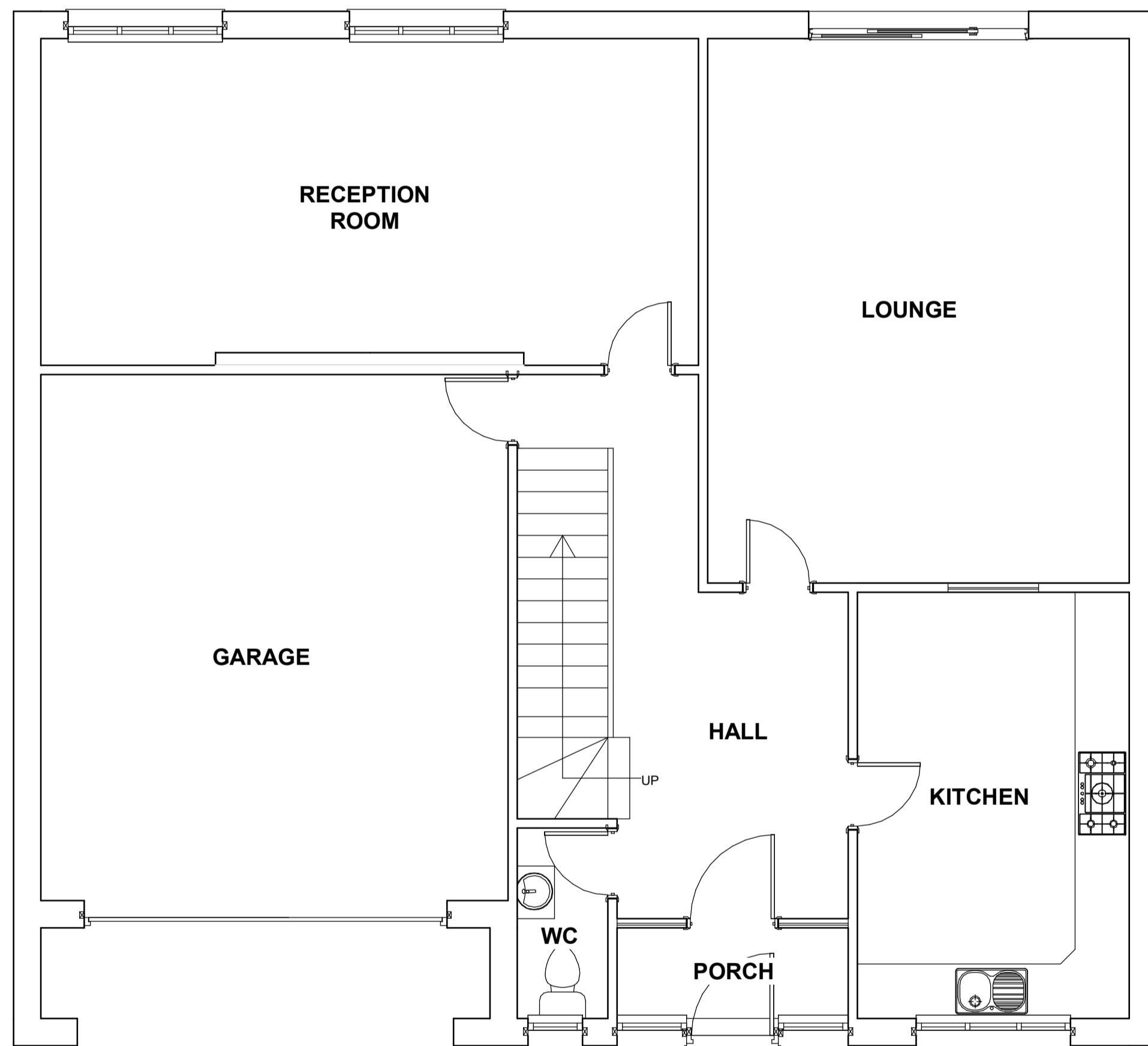
Existing Site / Ground Floor Layout 1 : 50
