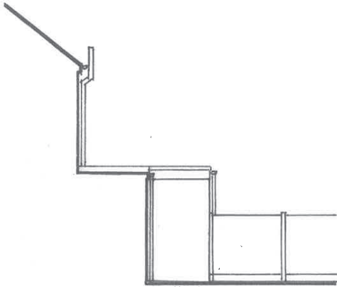
West / Side Elevation as existing scale: 1/100
