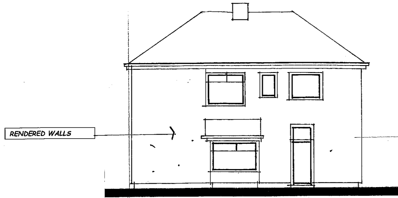
EXISTING REAR ELEVATION EAST 1:100
