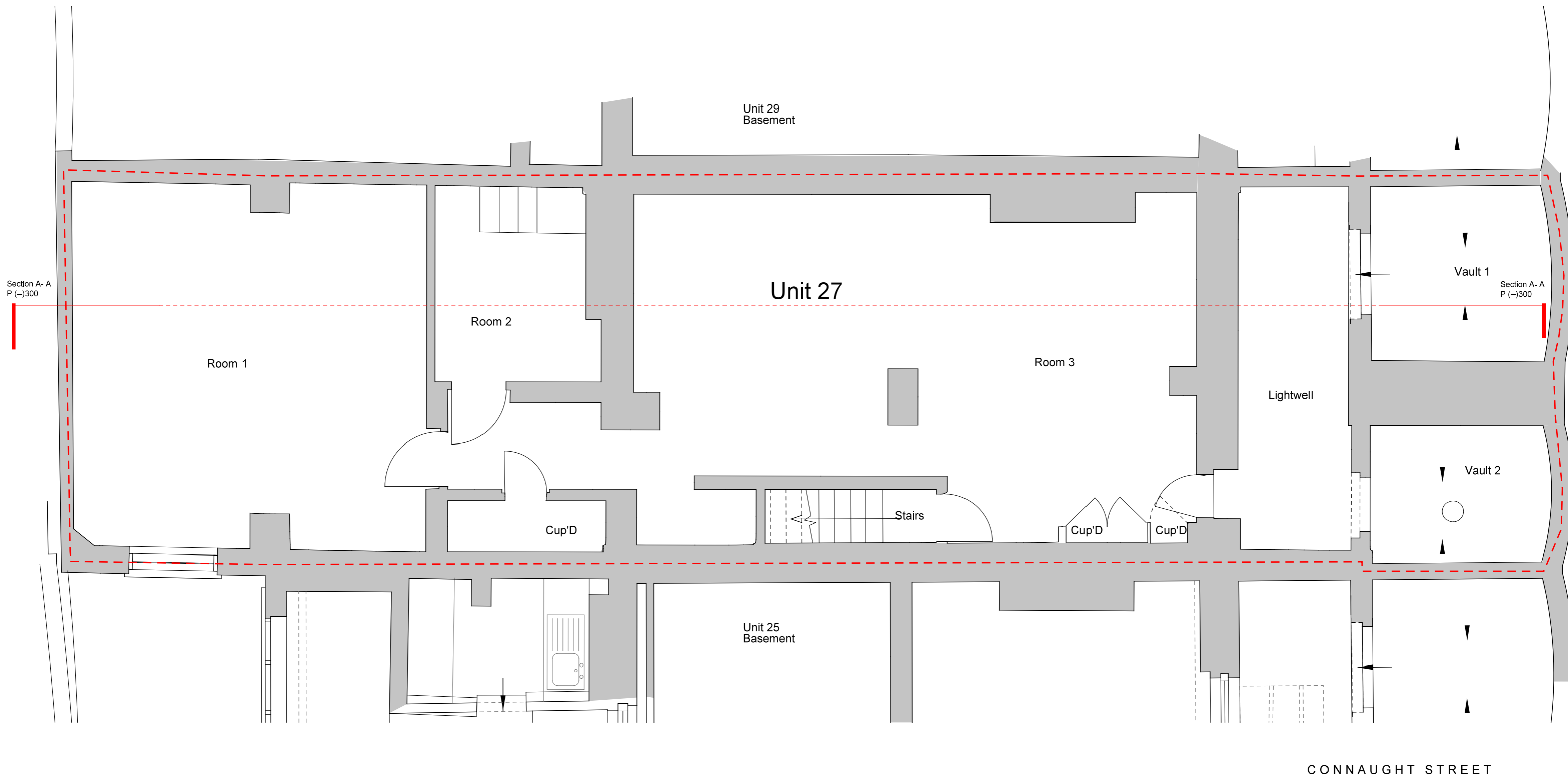
Existing Basement Floor Plan
