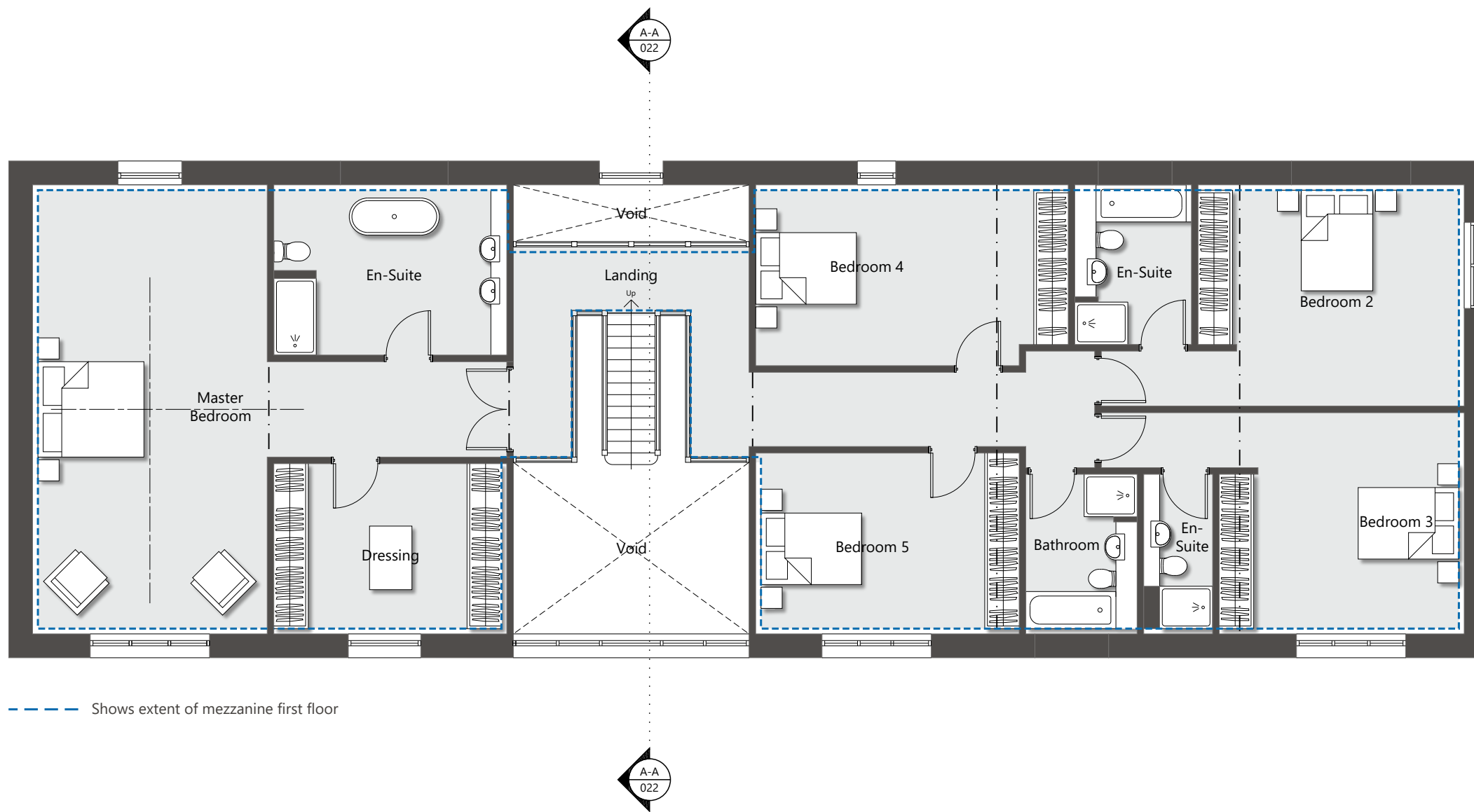
First Floor Plan Internal floor area 203m 2
