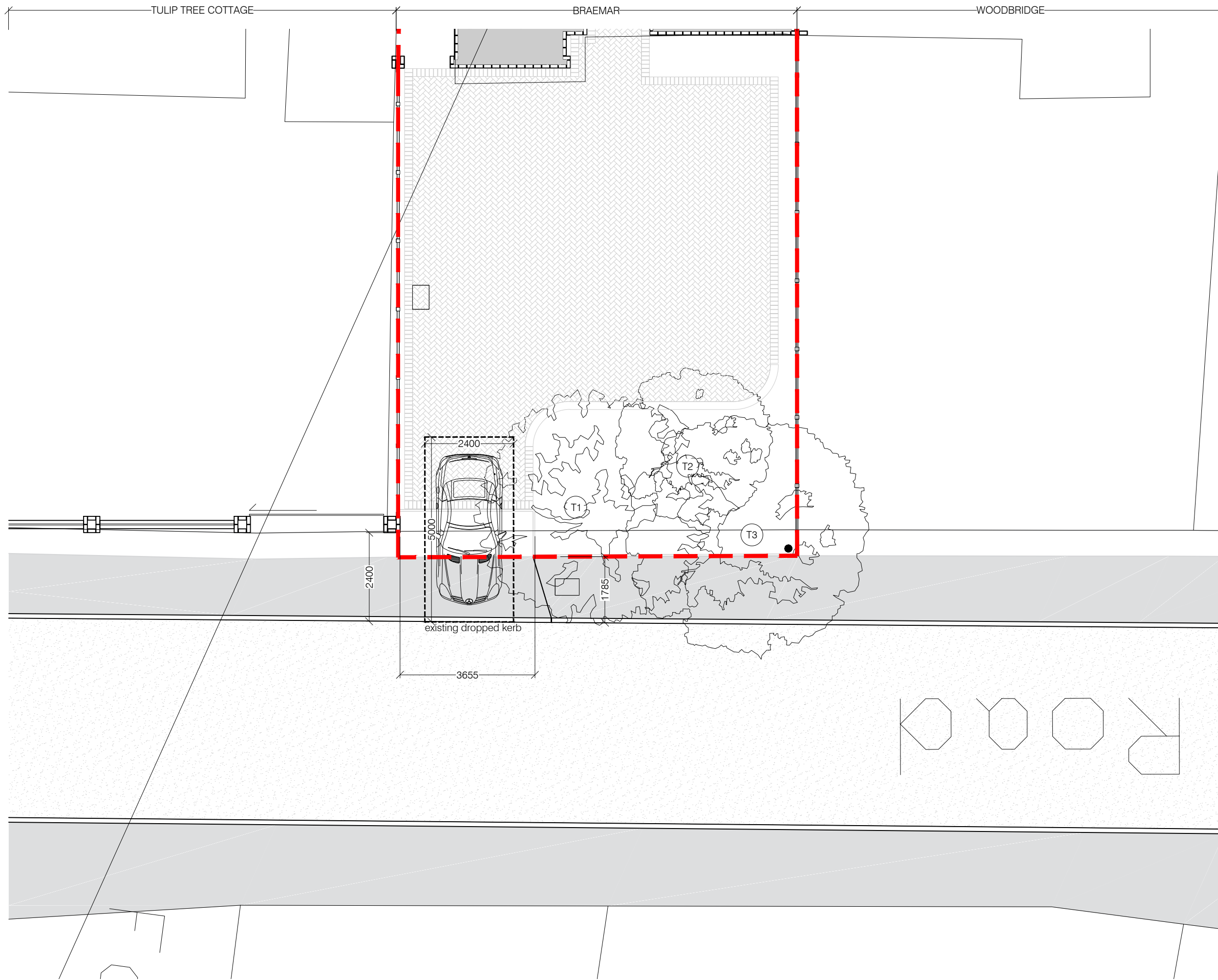
1 EXISTING DRIVEWAY PLAN 1:100 @ A3
