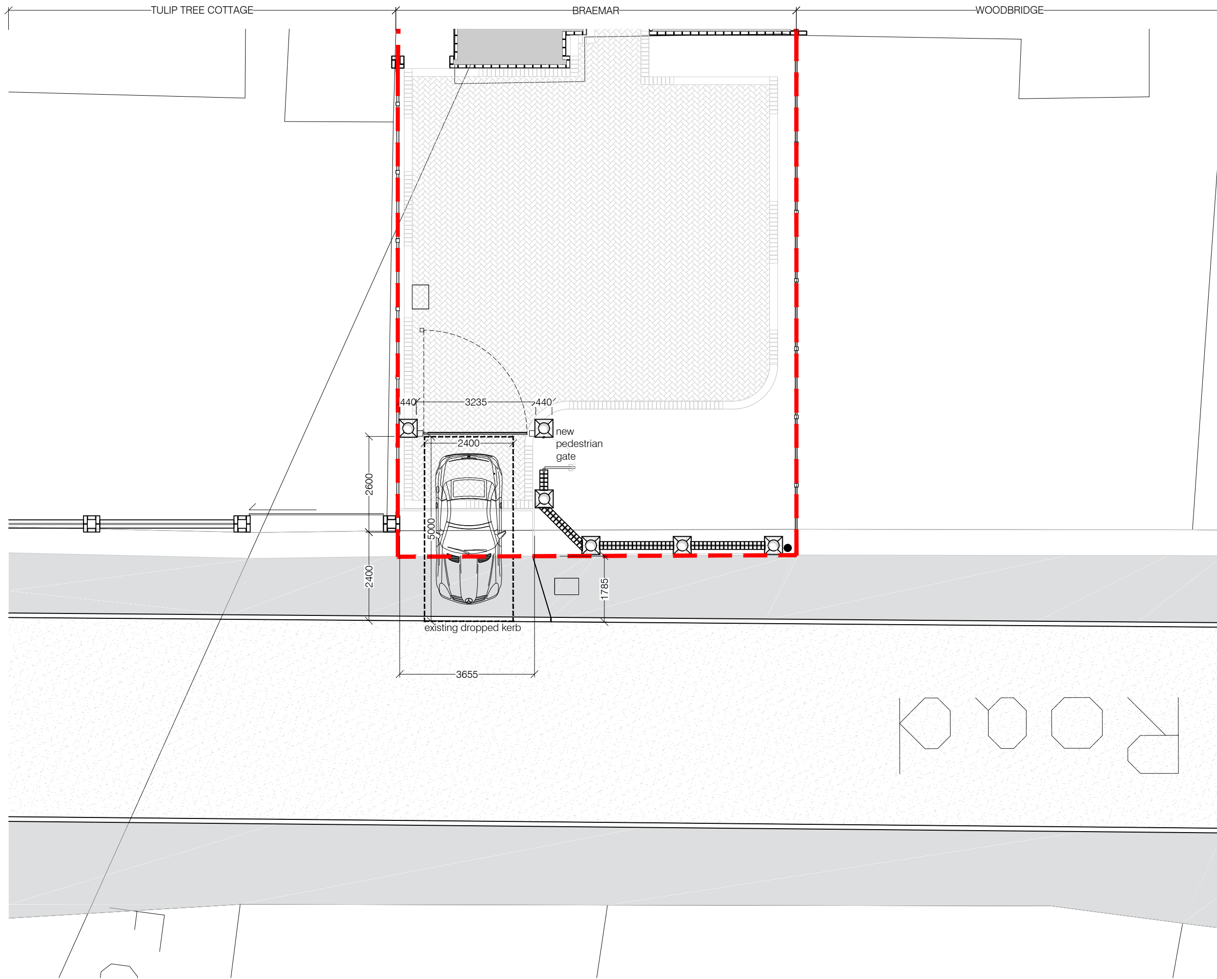
1 PROPOSED DRIVEWAY PLAN 1:100 @ A3
