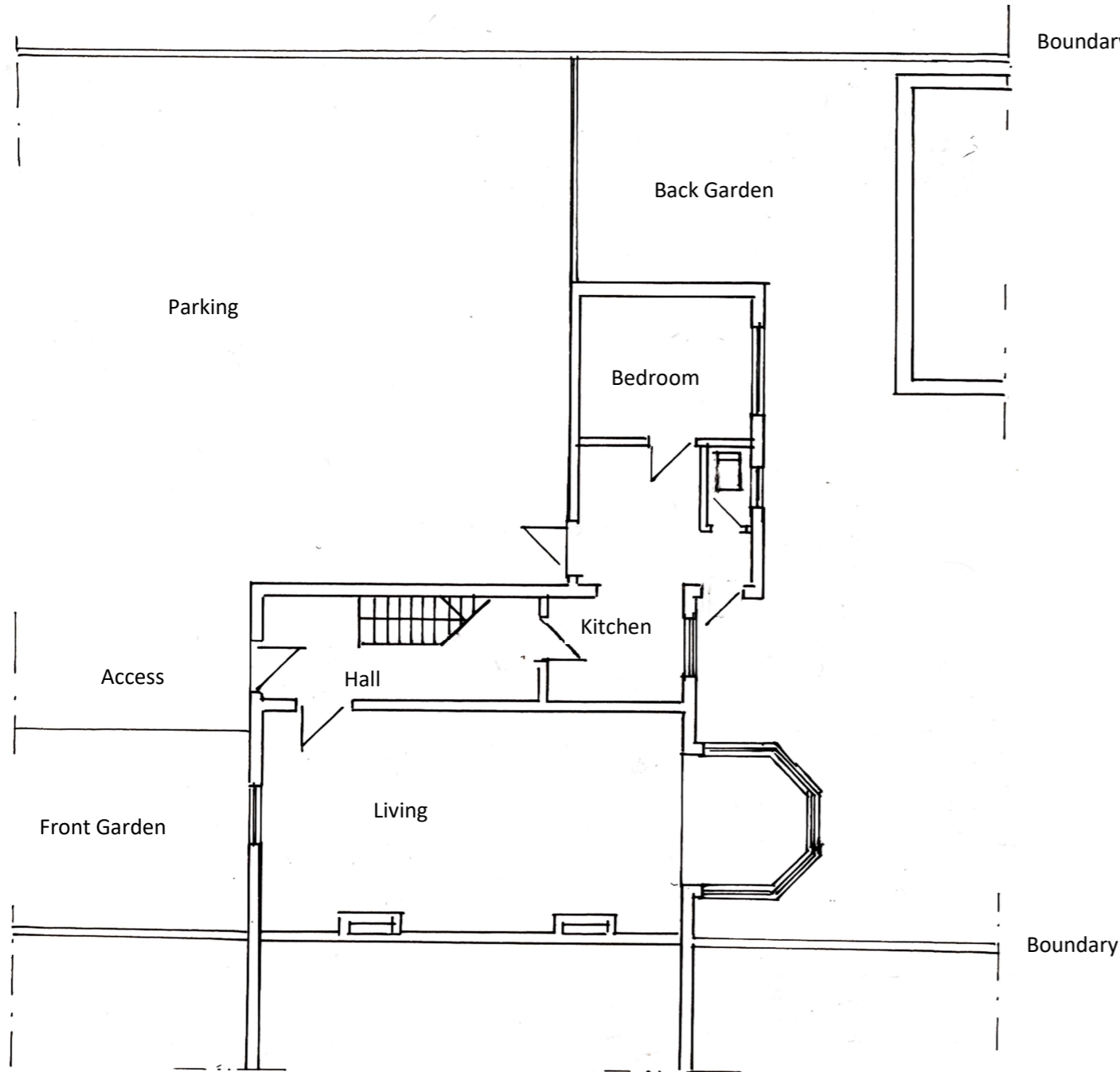
GROUND FLOOR
