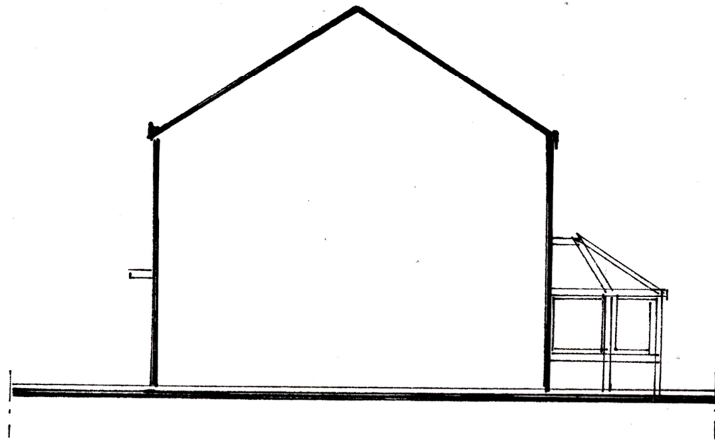
WEST ELEVATION
