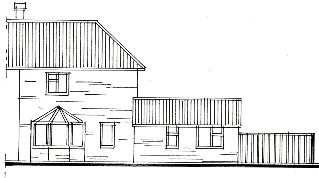
SOUTH ELEVATION
