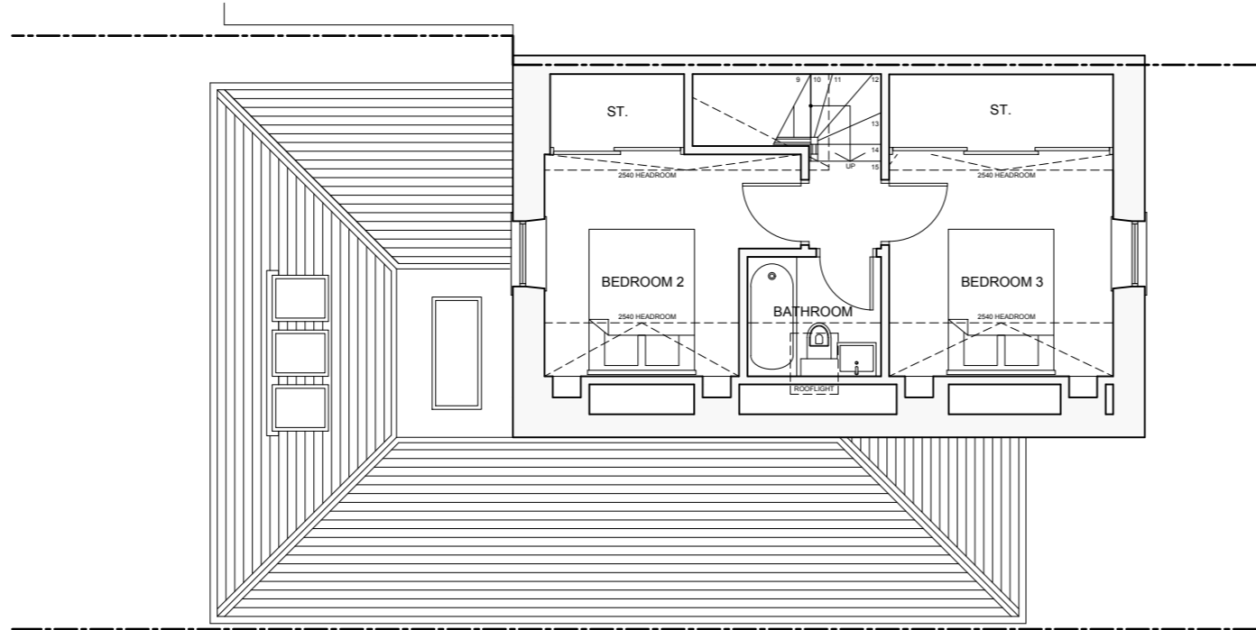
FIRST FLOORPLAN
