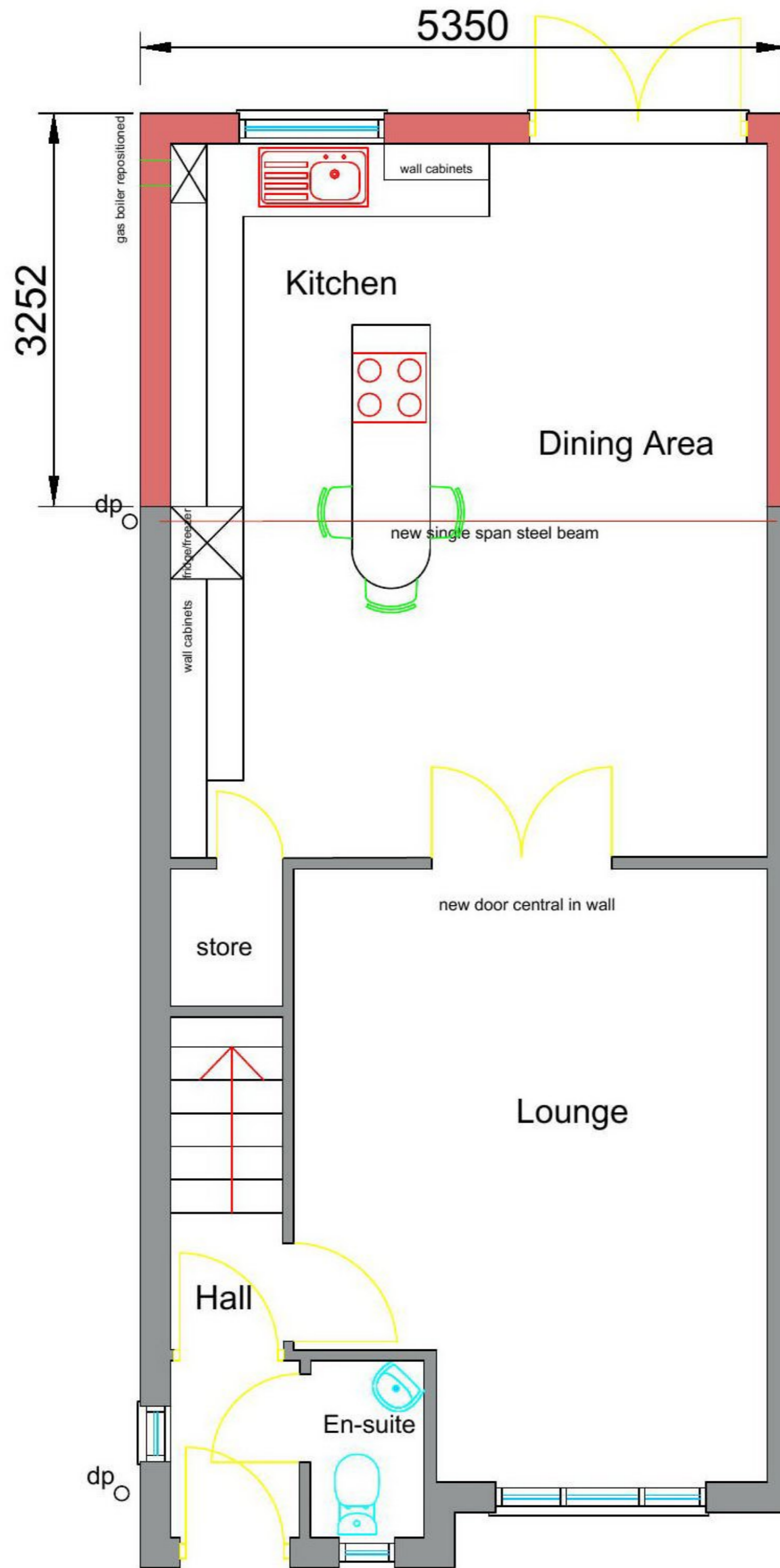
(0) Ground Floor Plan as Proposed 6 Levern Bridge Way G53 7AH 02 Scale 1:50 @ A3
