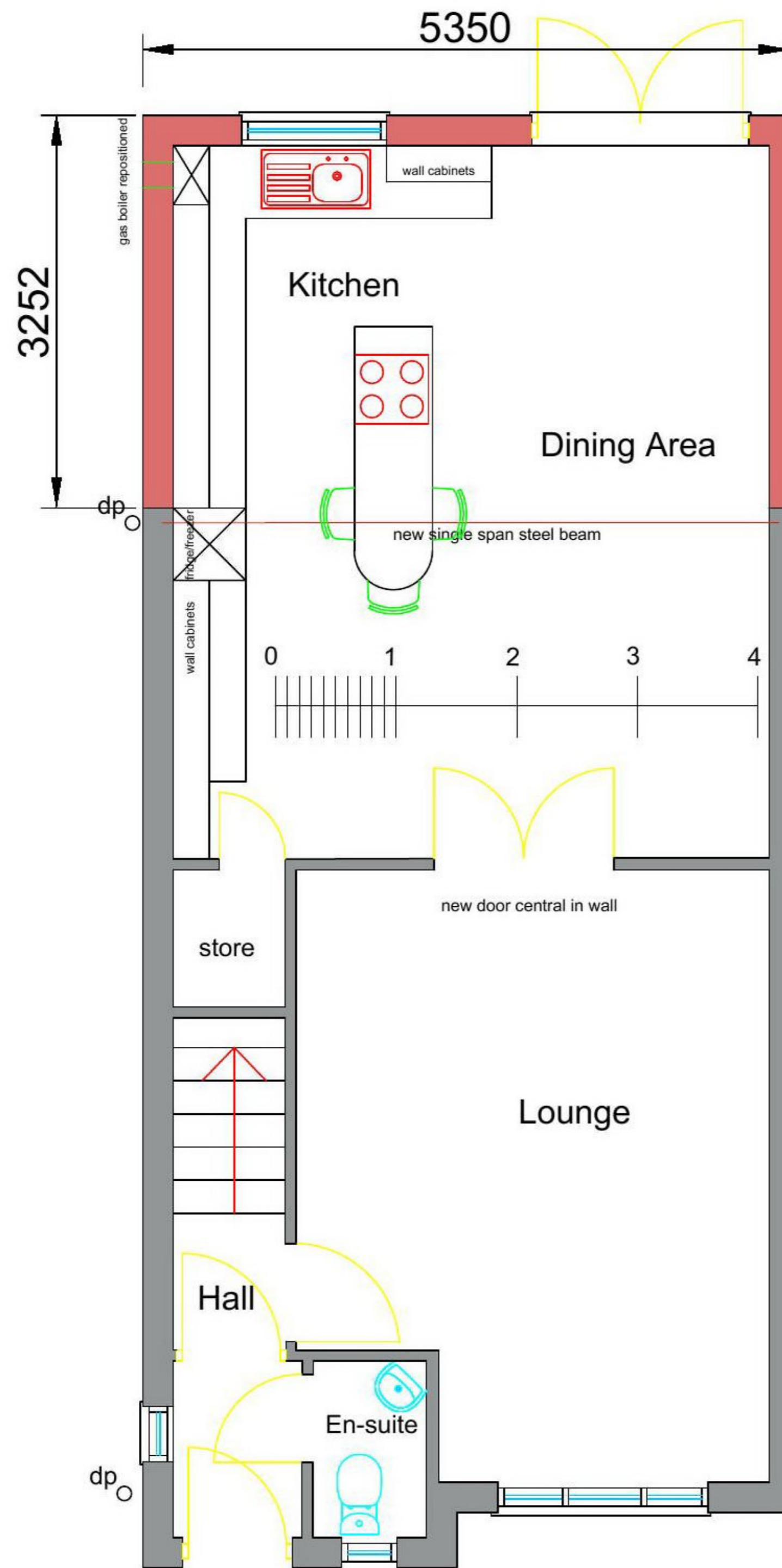
Ground Floor Plan as Proposed 6 Levern Bridge Way G53 7AH
