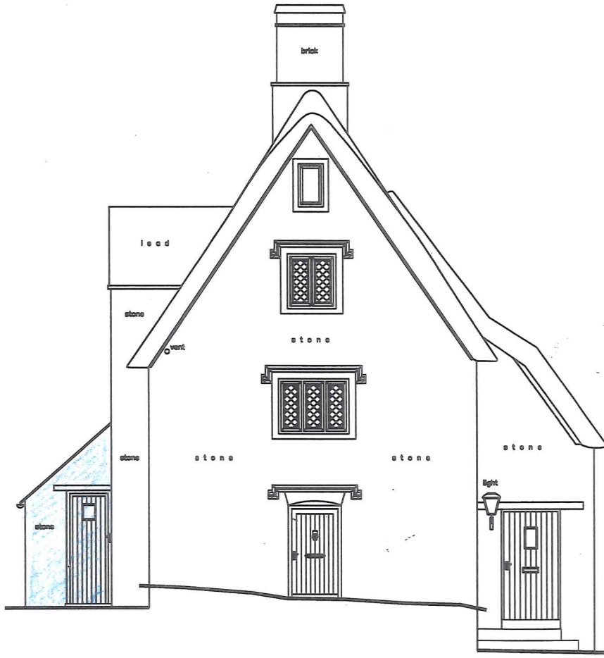
SOUTH EAST ELEVATION ( 98.00m—Above Assumed Datum )
