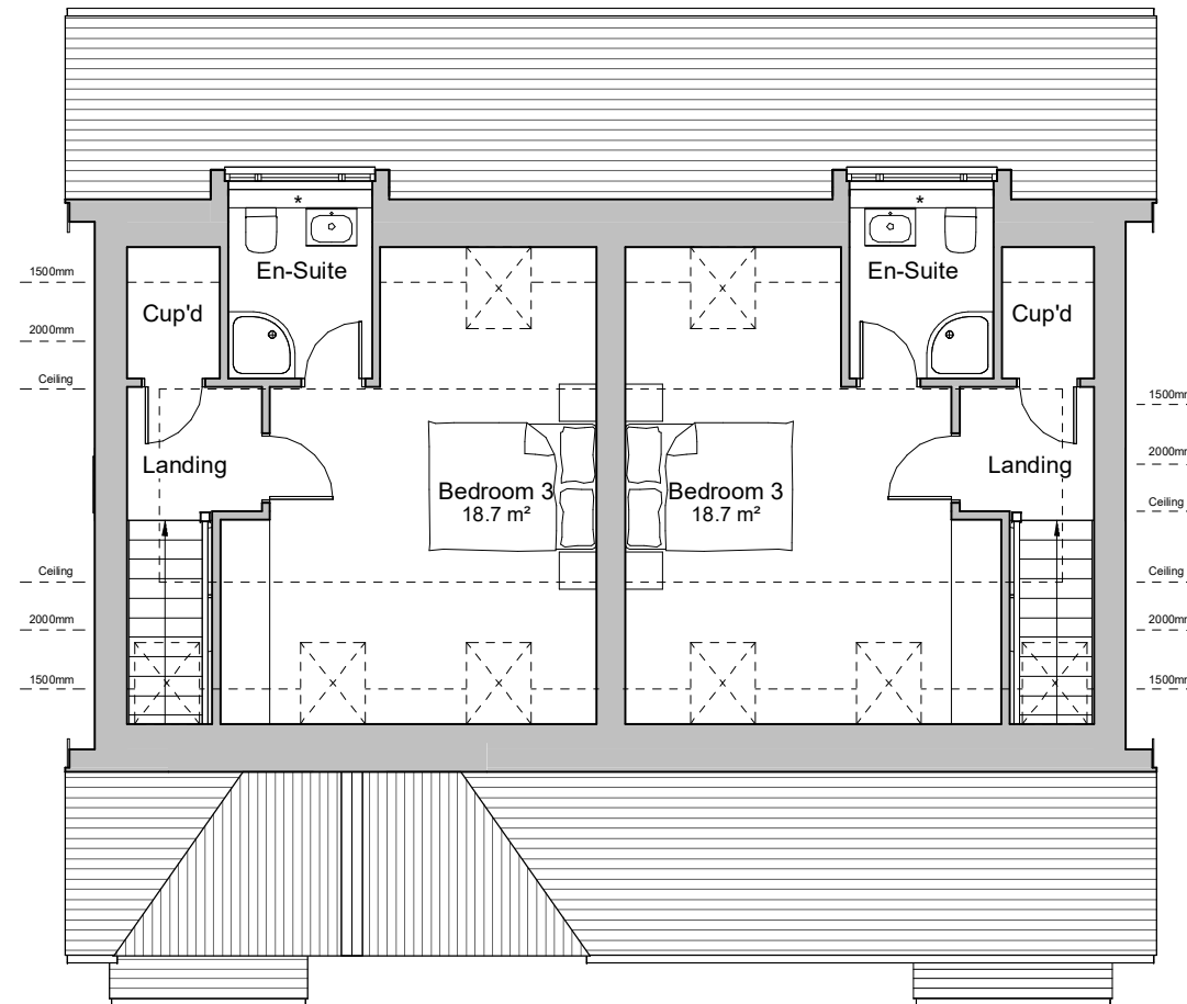
Plot 4 Second Floor Plan
