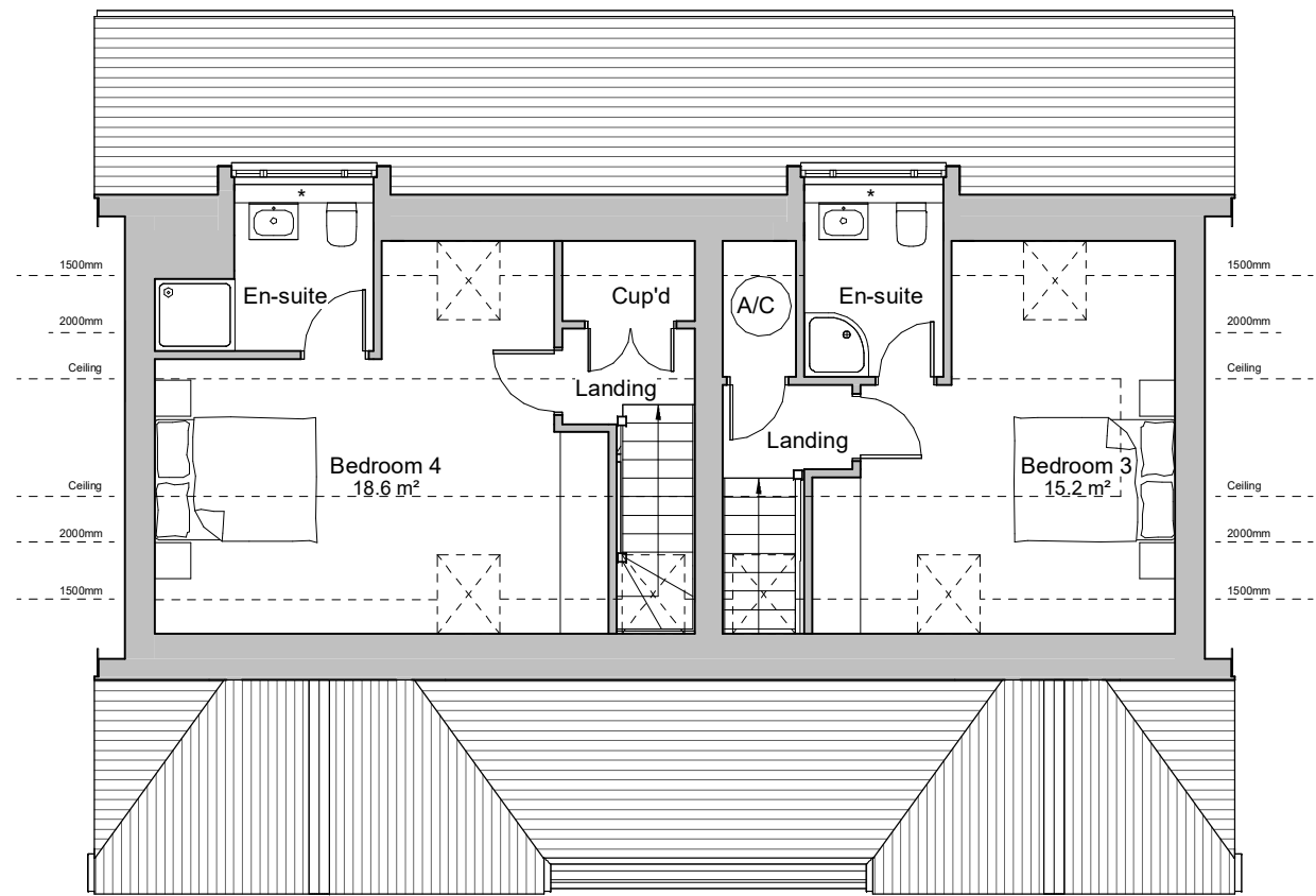
Plot 5 Second Floor Plan
