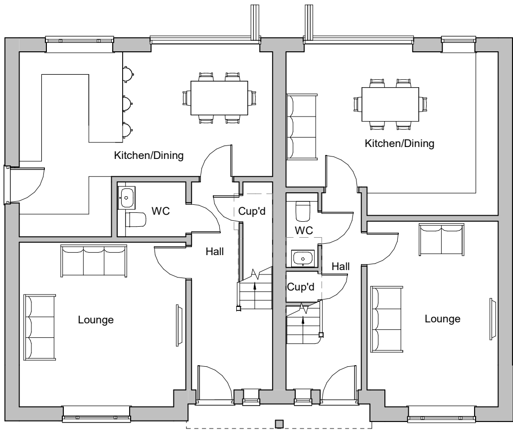
Plot 5 Ground Floor Plan
