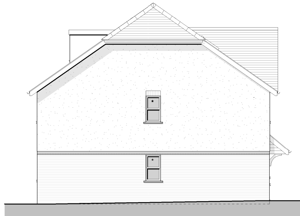
Plot 4 Left Elevation
