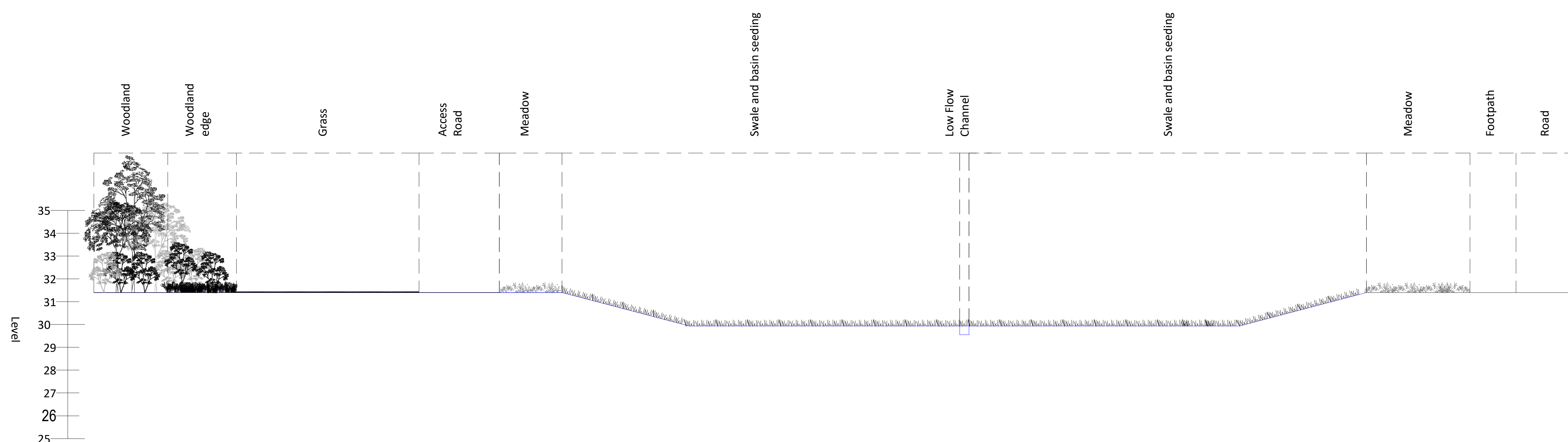
SUDS Basin Section 2 1 : 100
