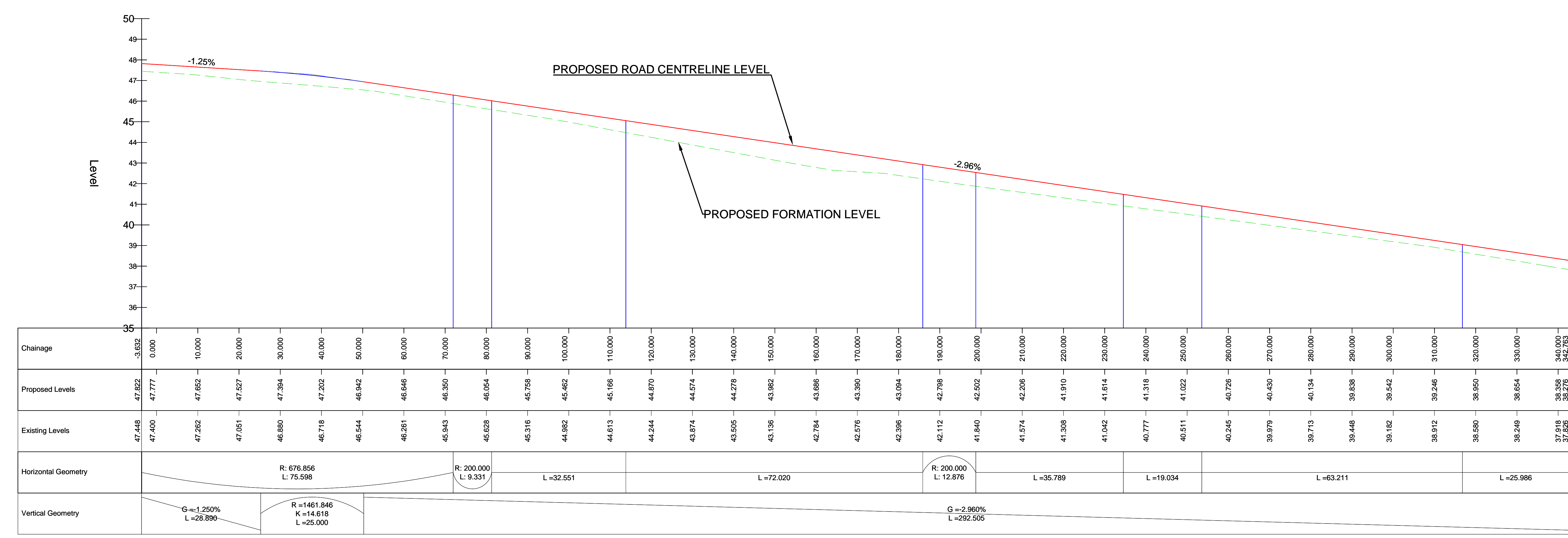
PROPOSED PH2 - RD 6 - LONGSECTION SCALE: H 1:500, V 1:100. DATUM: 35.000
