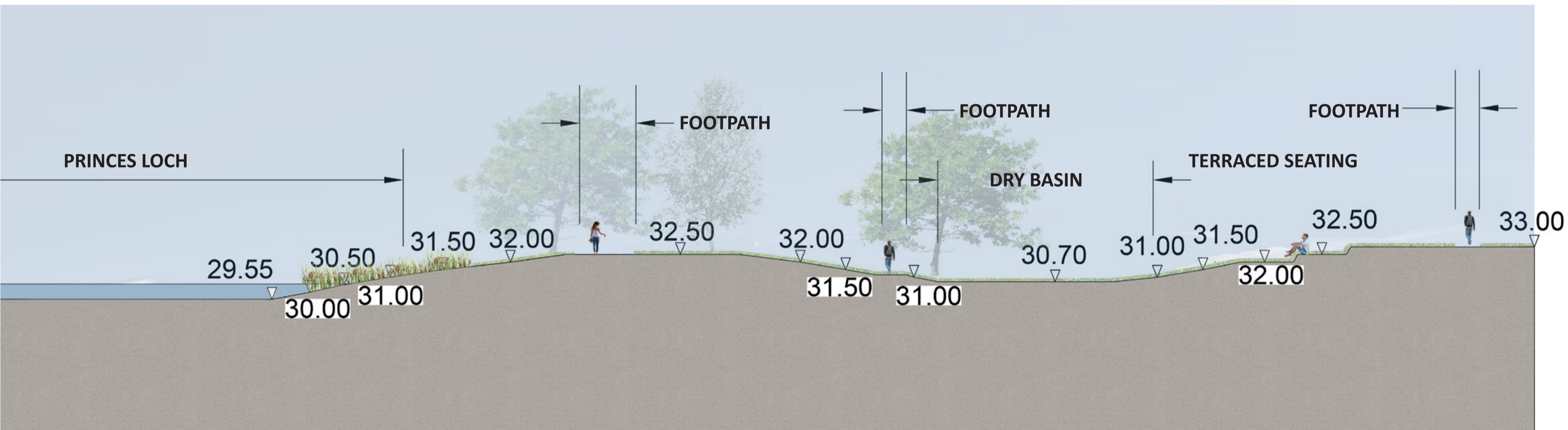
SITE SECTION AA SCALE 1:200
