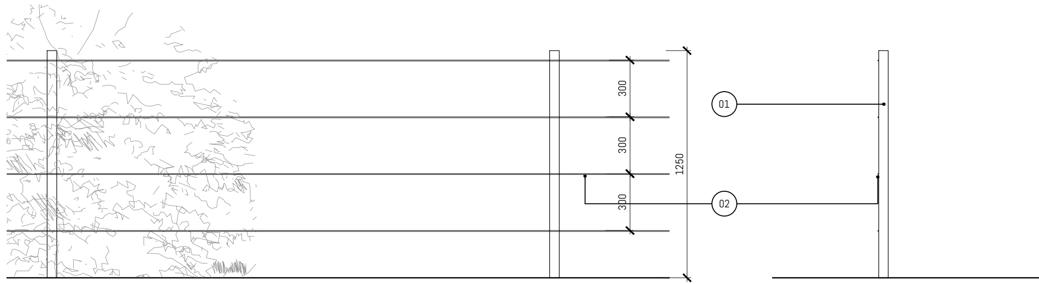
PL-010 ELEVATION 2 1:20 A3 SCALE
