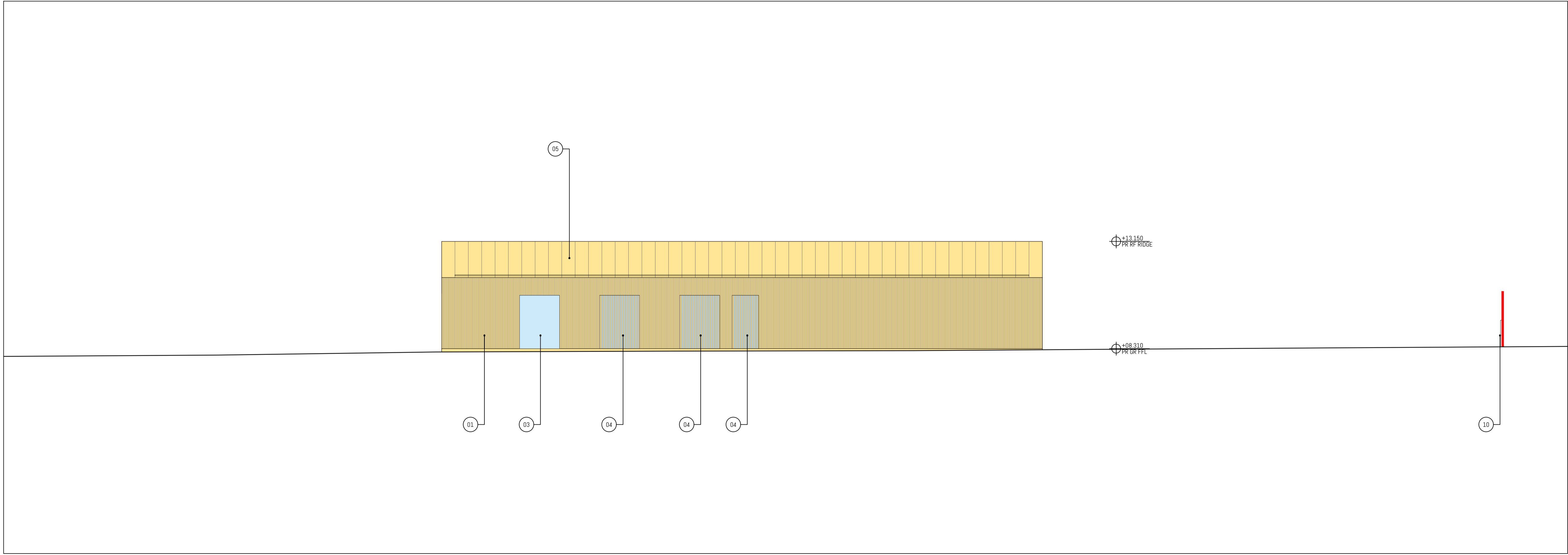
039-PL-006 PROPOSED / ELEVATION / EAST 2 1:100 A1 / 1:200 A3 SCALE
