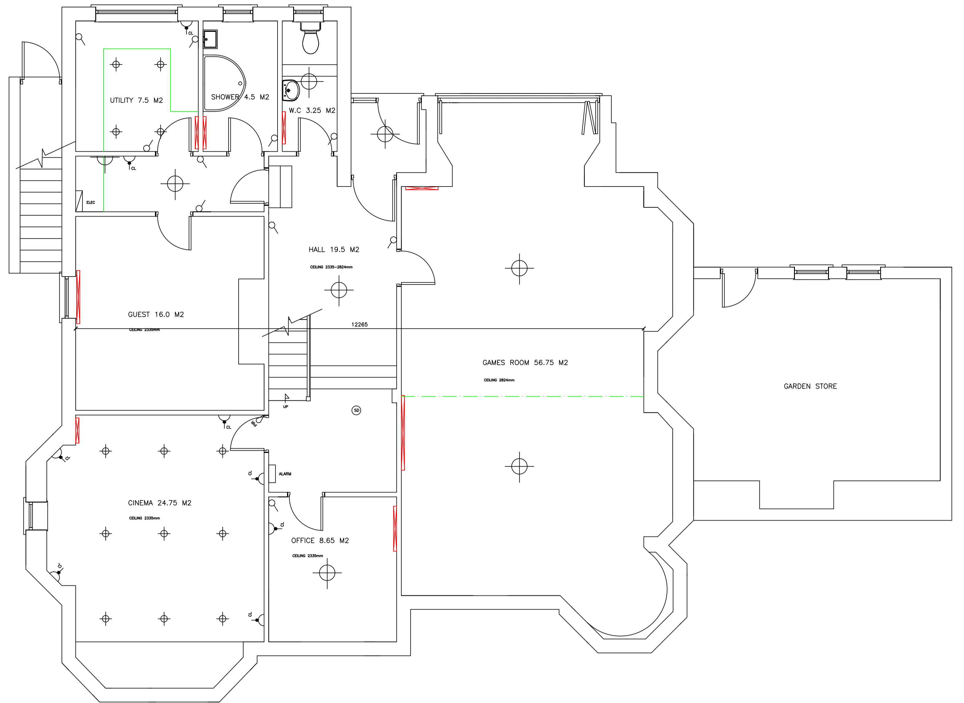
EXISTING BASEMENT FLOOR LAYOUT PLAN (SCALE 1:50)
