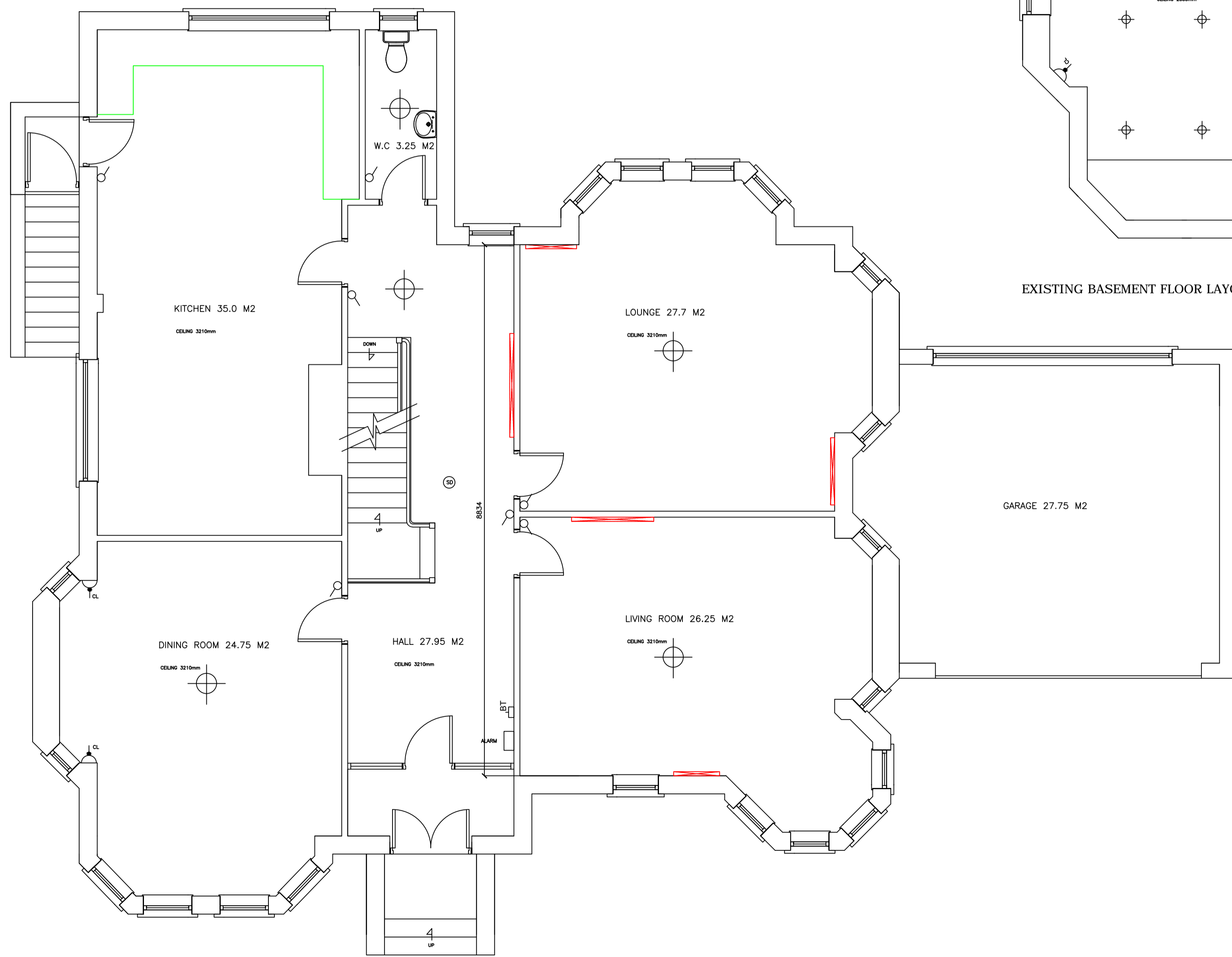
EXISTING GROUND FLOOR LAYOUT PLAN (SCALE 1:50)
