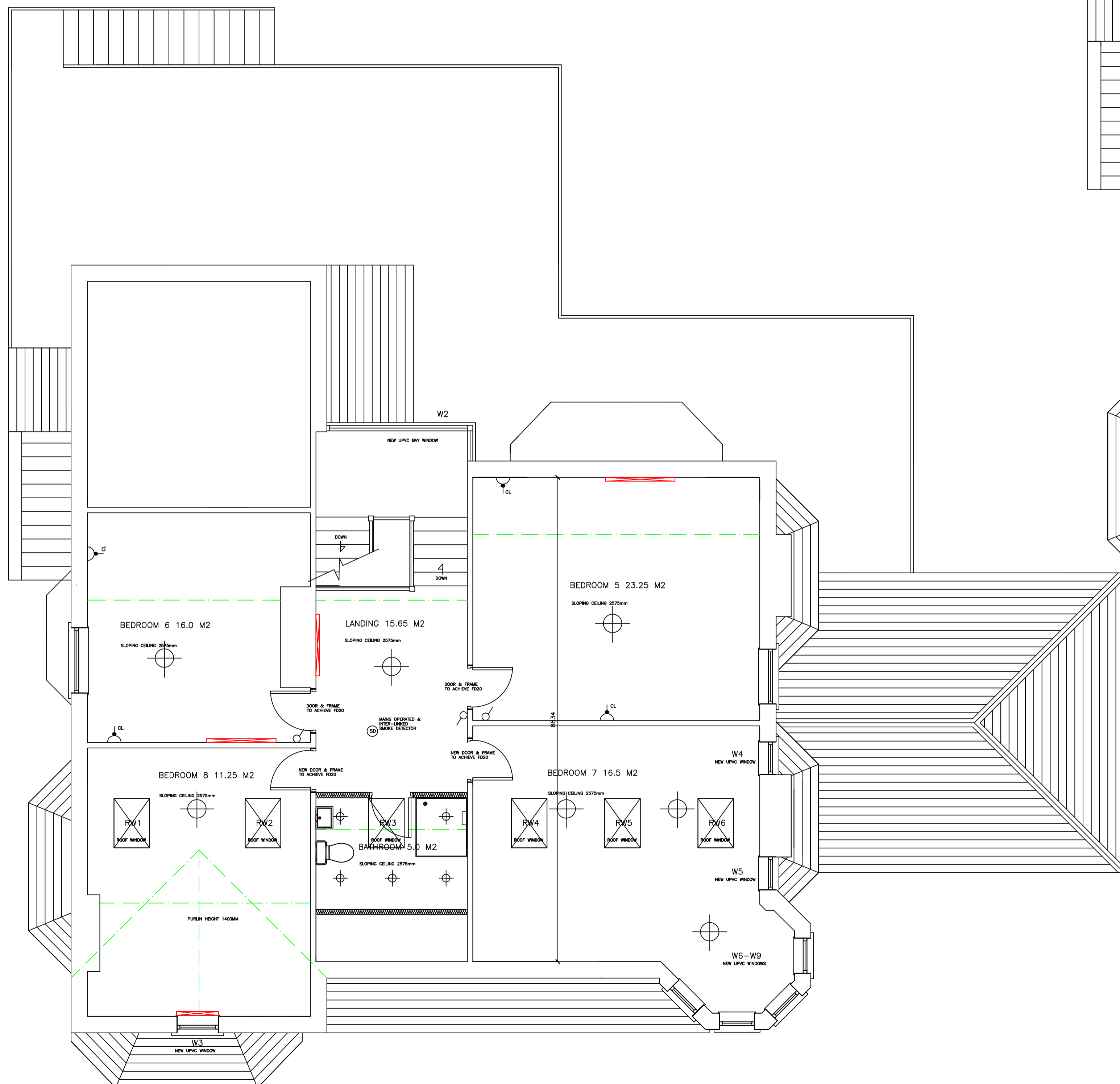
PROPOSED SECOND FLOOR LAYOUT PLAN (SCALE 1:50)
