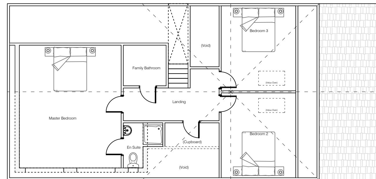
Proposed First Floor Plan (1:50)
