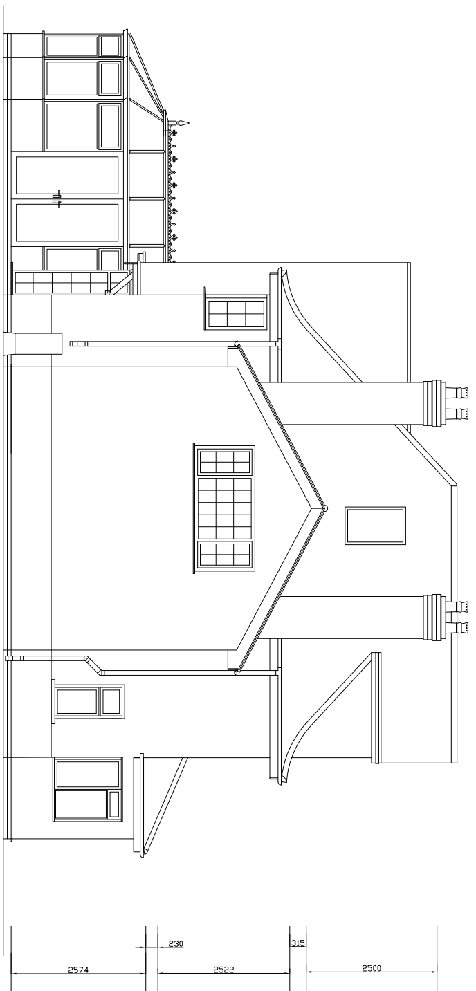
Side Elevation (West)
