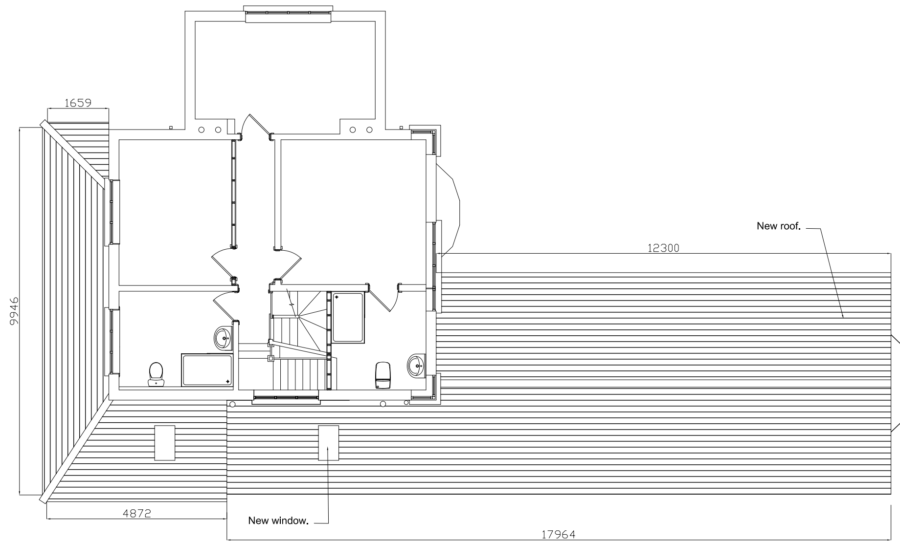
First Floor & Extension Roof
