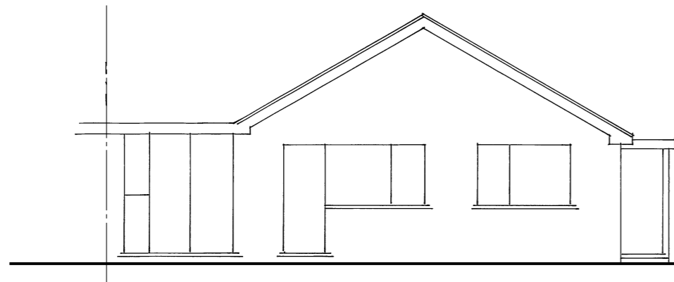
Proposed NW/Rear Elevation
