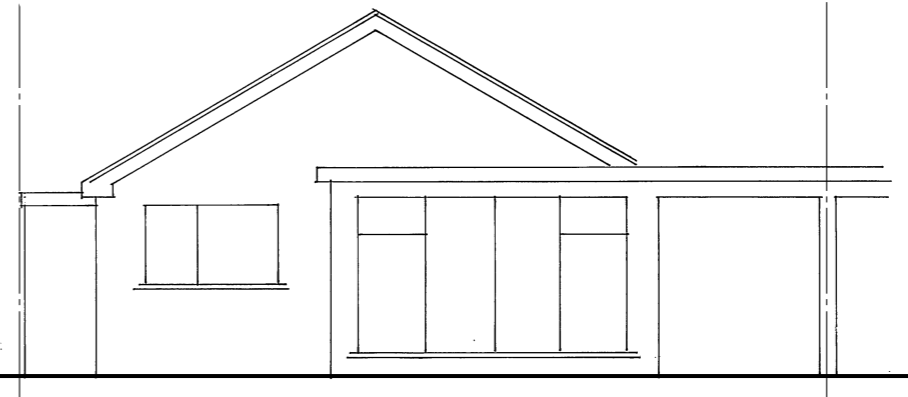
Proposed SE/Front Elevation
