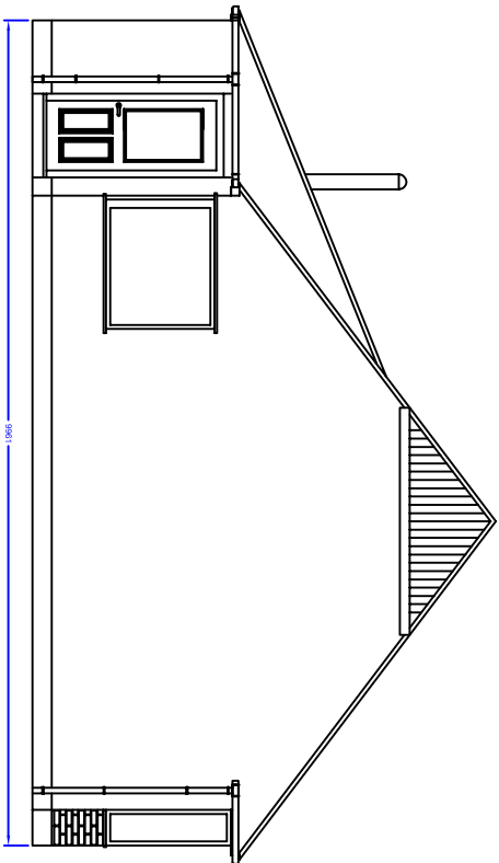
Existing Side View
