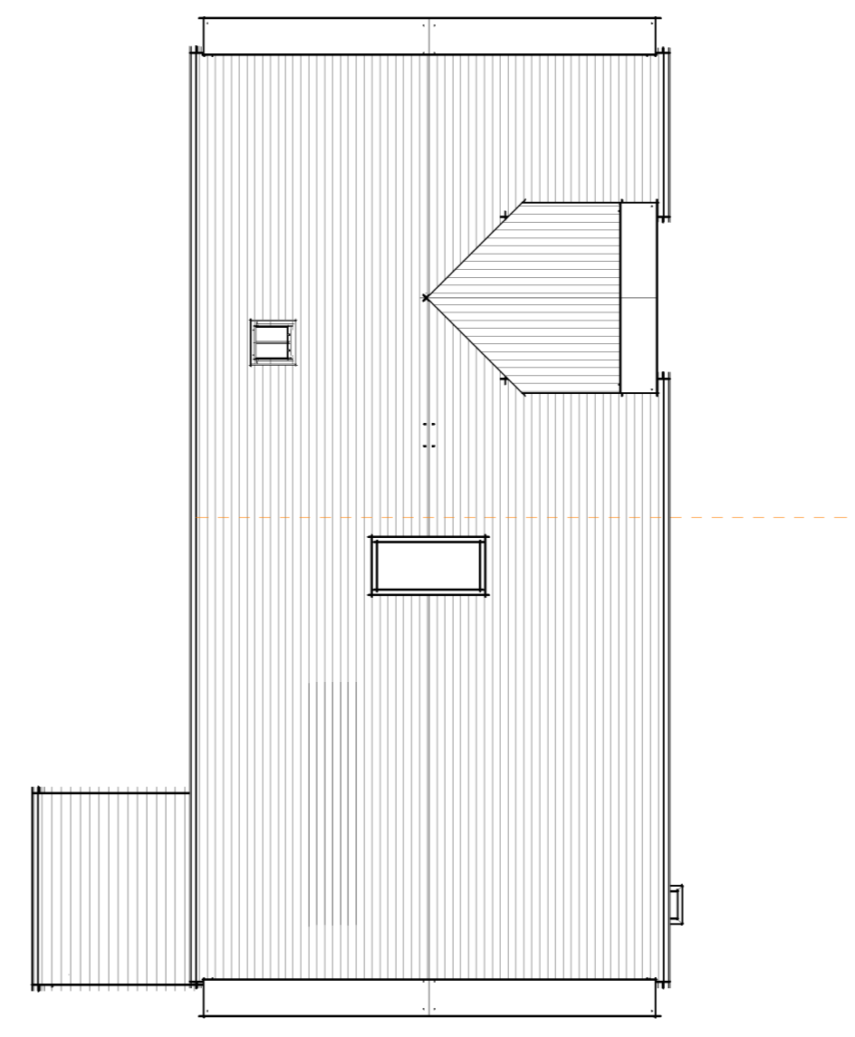
2 1.3 Existing Roof Plan 1:100
