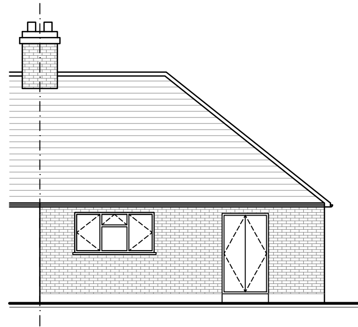
2 EXISTING REAR ELEVATION
