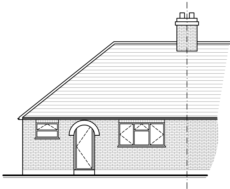
1 EXISTING FRONT ELEVATION
