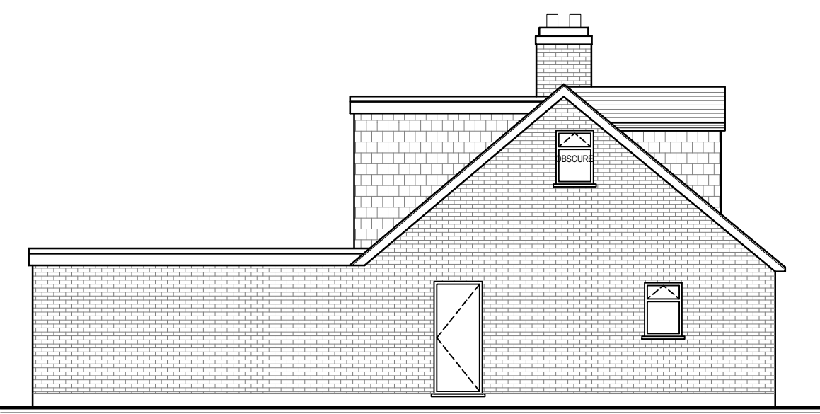
3 PROPOSED LEFTSIDE ELEVATION
