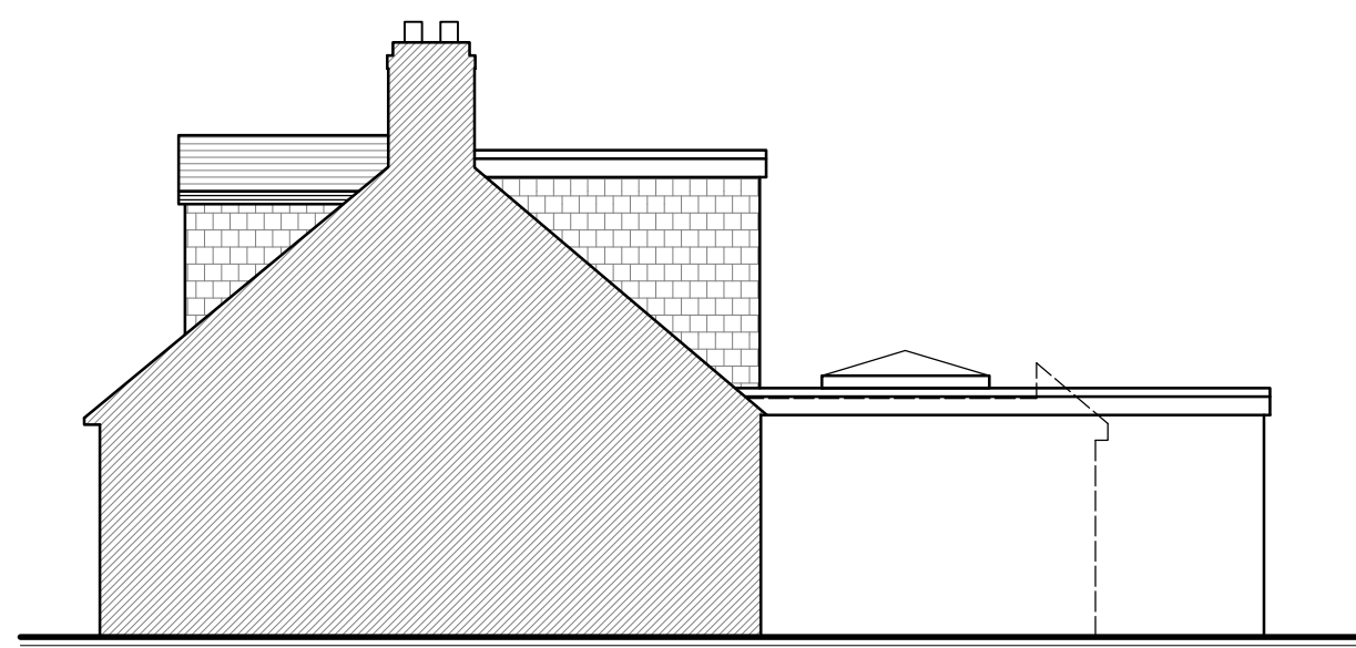
4 PROPOSED RIGHTSIDE ELEVATION
