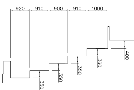
SECTION VIEW ON ROW DEPTH & RISE Scale 1:50
