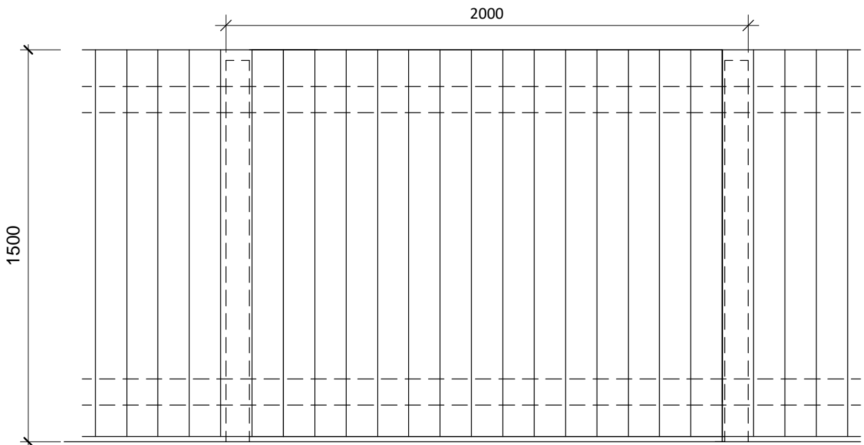
1500mm high feather edge timber fence on timber posts. All timbers to be treated softwood
