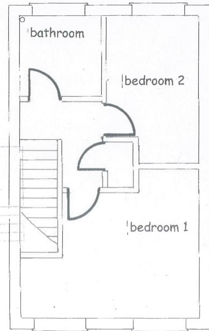
Ex First Floor Plan
