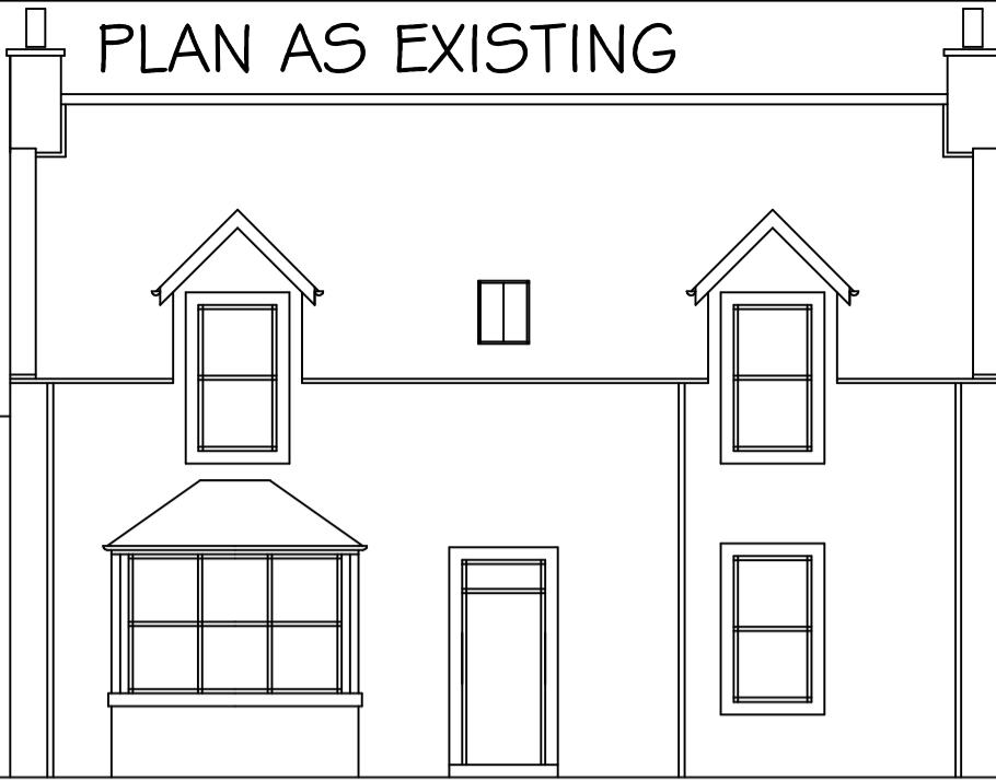
FRONT ELEVATION 1:100
