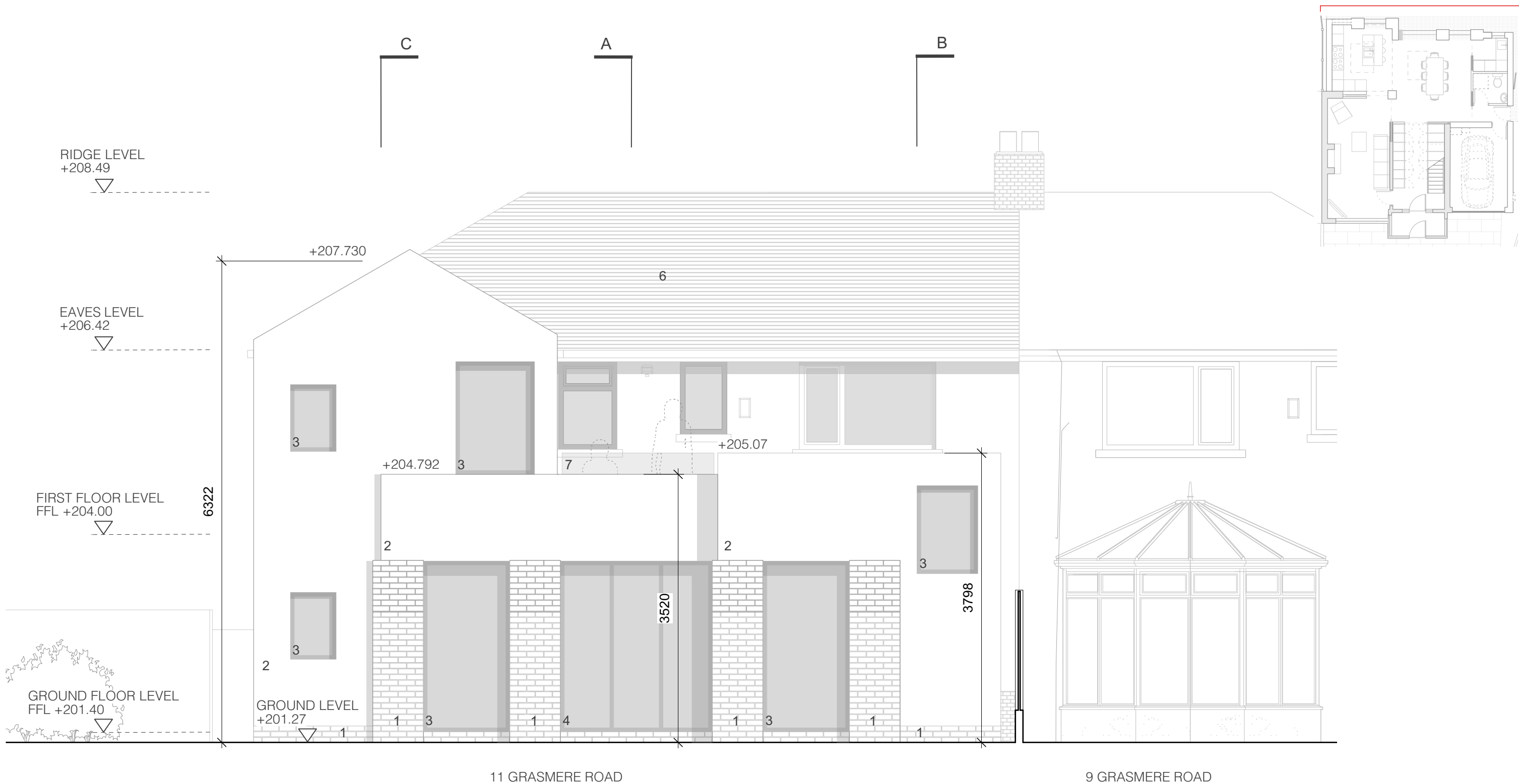
2 PROPOSED EAST ELEVATION 1:50 (A3)
